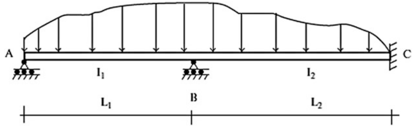
Fig. 10.21 Two-span beam with a moment release at a support
