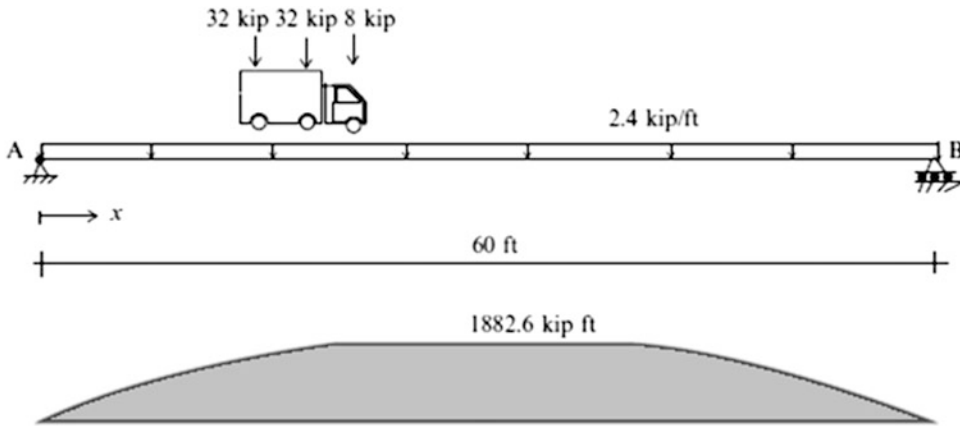
Fig. E3.30e Discrete moment envelope for the combined (dead + truck) loading
