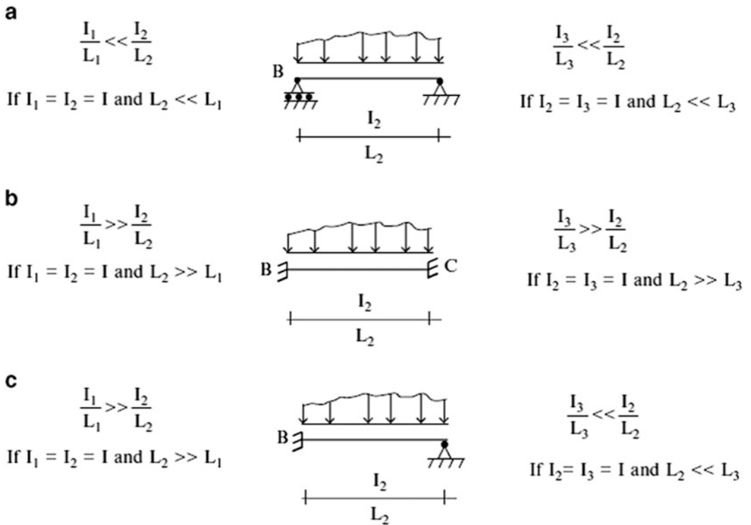
Fig. 11.5 Summary of approximate models for extreme values of L_1/L_2 and L_3/L_2 . (a) Hinged model. (b) Clamped end model. (c) Clamped/hinged model
