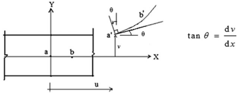
Fig. 3.19 Definition of displacement components
