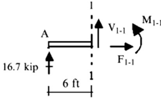
Fig. E1.3c Left segment-cutting plane 1-1
