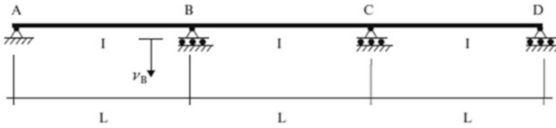
Fig. E10.5c Settlement at B
