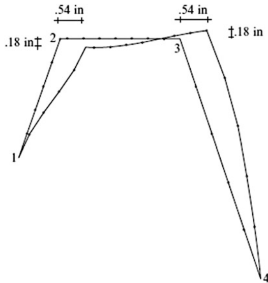
Fig. E10.19c Deflection profile— I = 200 \text{ in.}^4
