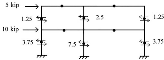
Fig. E11.2b Shear distribution for the columns (kip)
