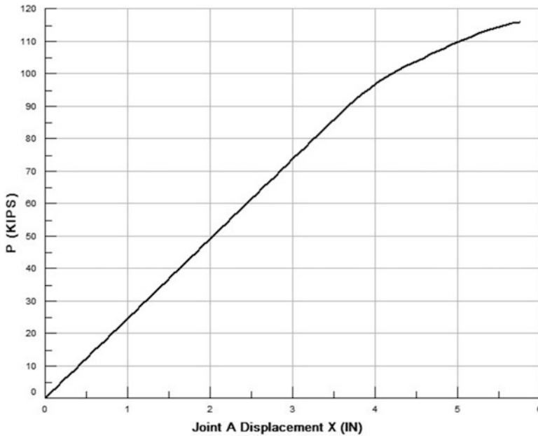
Fig. E16.7b Pushover results, P vs. joint displacement
