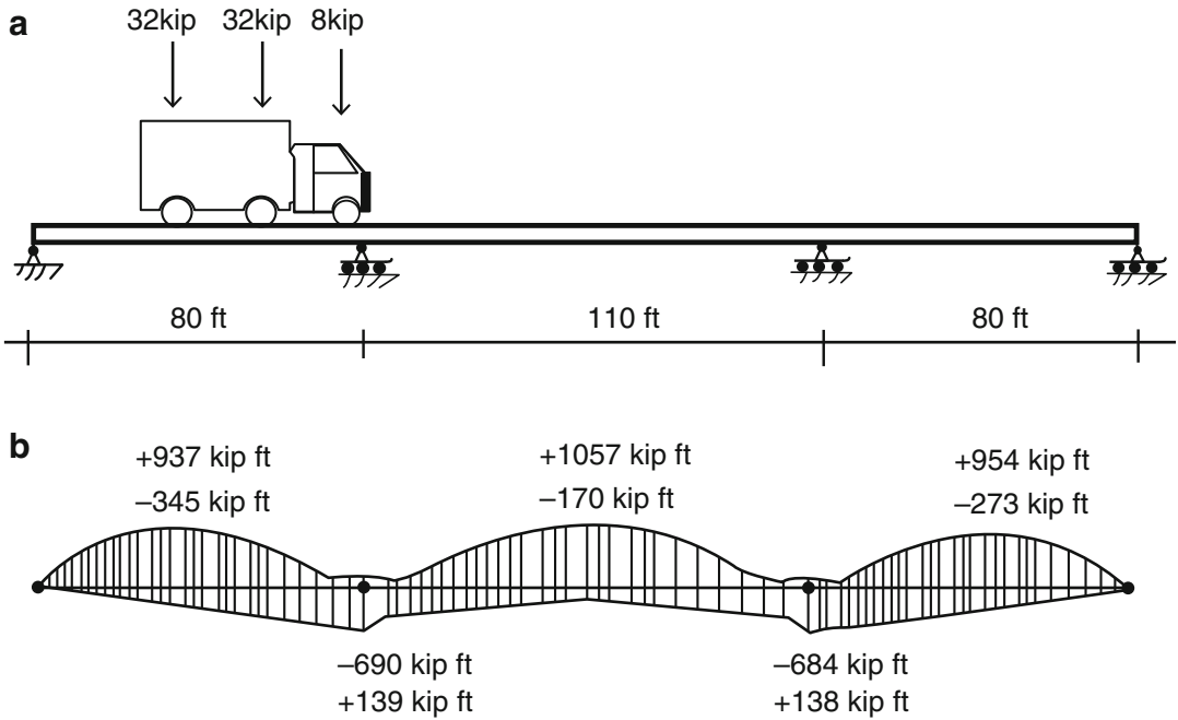
Fig. 13.33 Force envelopes—three-span girder. (a) Geometry and loading. (b) Moment envelope
