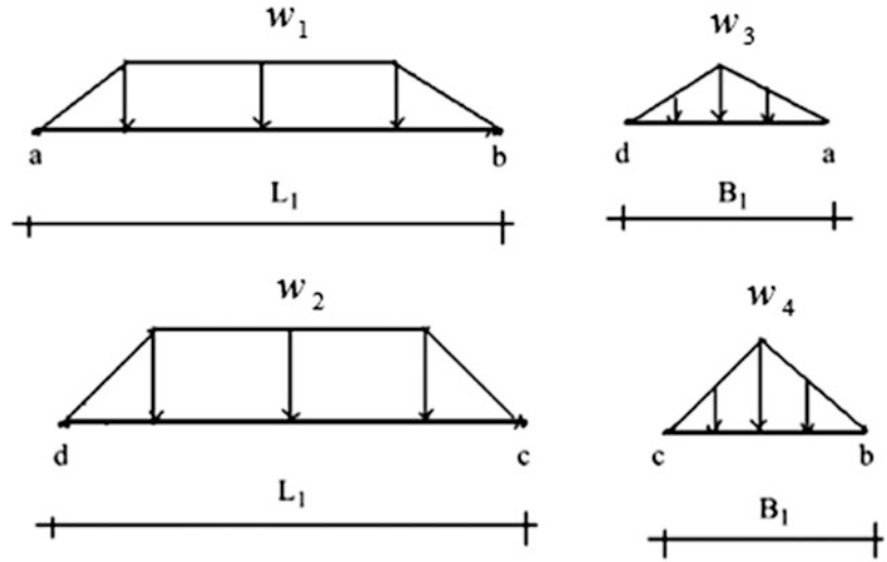
Fig. 15.5 Two-way action perimeter beam loadings for uniform floor loading—panel abcd
