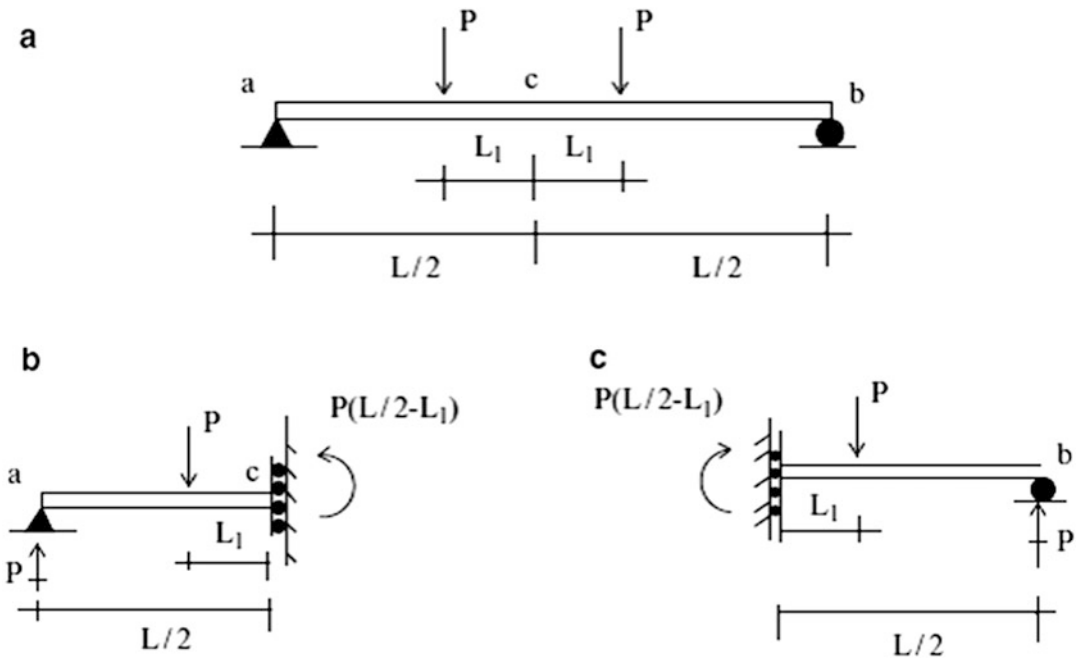
Fig. 3.48 Boundary conditions on symmetry axis—symmetrical planar loading. (a) Symmetrical load. (b) Left segment. (c) Right segment
