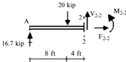
Fig. E1.3d Left segment-cutting plane 2-2
