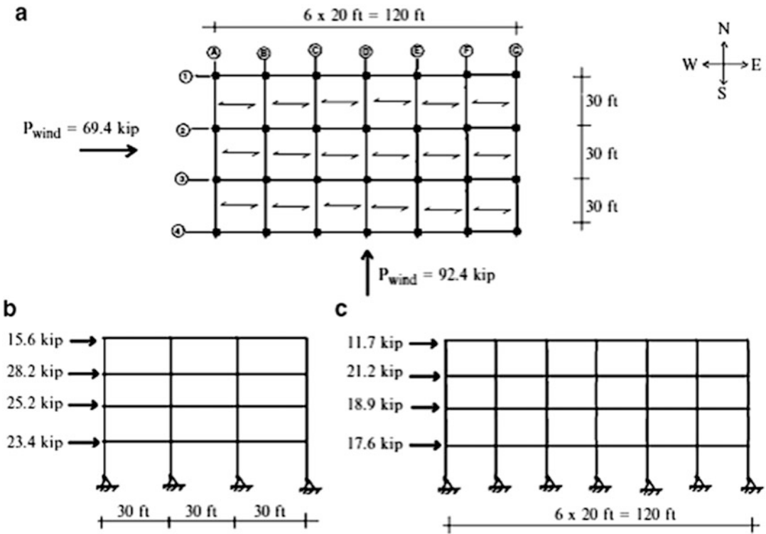
Fig. 15.15 Global Wind loads. (a) Plan. (b) N-S. (c) E-W
