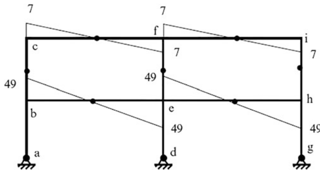
Fig. E11.1e Bending moment distribution for the beams (kN m)
