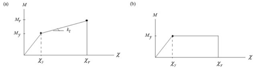
Fig. 16.6 Bilinear moment–curvature models. (a) General bilinear model and (b) EPPF model
