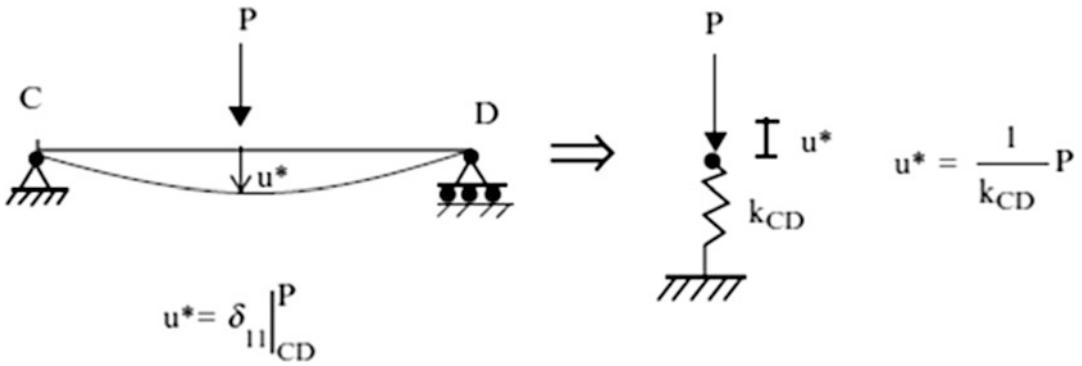
Fig. 9.20 Equivalent spring
