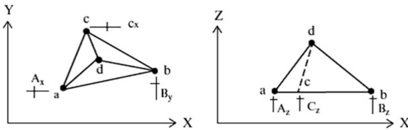
Fig. E2.21f Alternative restraint scheme #1
