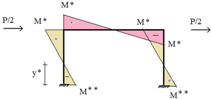
Fig. 9.46 Bending moment distribution—anti-symmetric loading
