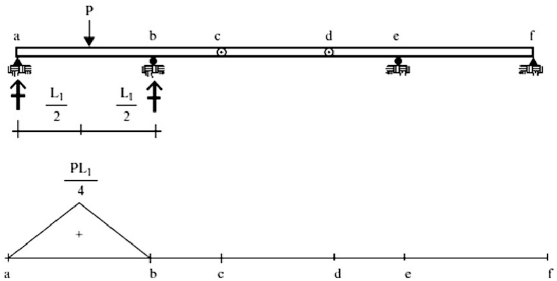
Fig. E3.27b Moment diagram—load on member AB
