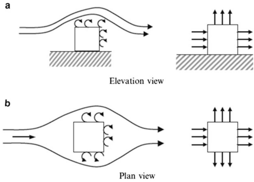
Fig. 1.11 Flow lines and pressure distributions due to wind
