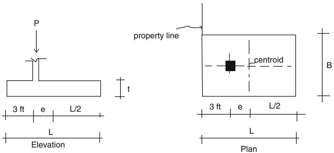
Fig. E7.2c Geometry and loading
