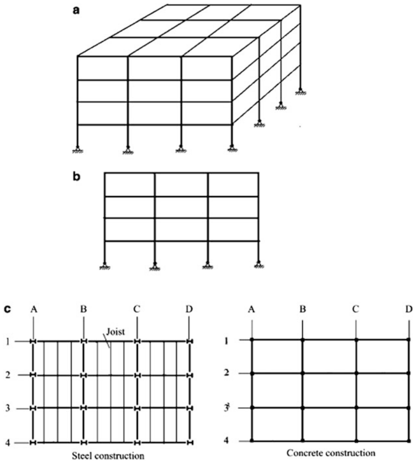
Fig. 15.2 Rectangular building. (a) Building frame. (b) Elevation view—individual frame. (c) Typical plan view—flooring system
