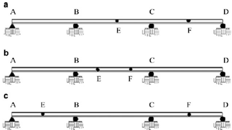
Fig. 3.11 Statically determinate versions of three-span beam with moment releases
