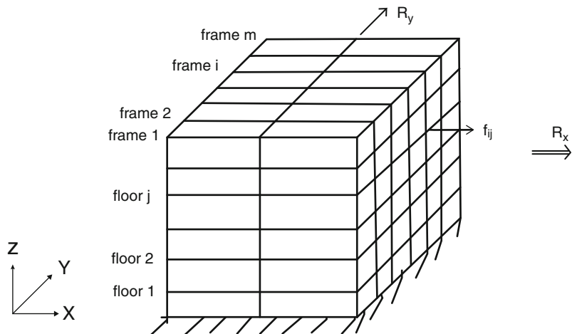
Fig. 14.4 Resultant force components
