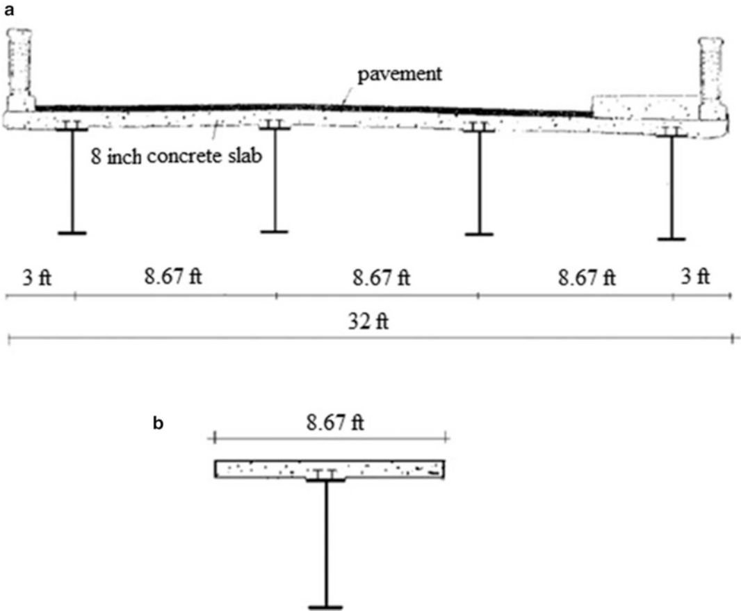
Fig. 13.18 (a) Cross section—bridge deck. (b) Cross section of single composite beam
