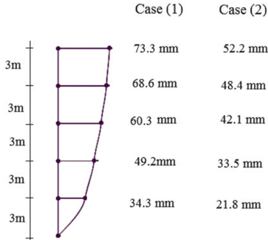
Fig. E15.2g Lateral displacement of the floors—earthquake
