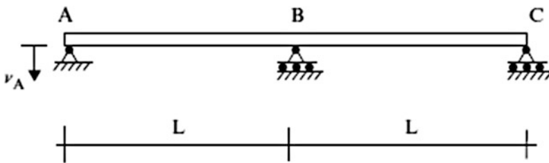
Fig. E10.2c Settlement at A
