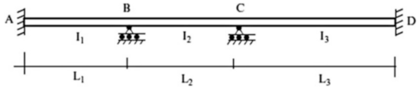
Fig. 10.22 Three span beam
