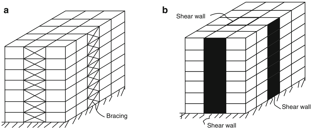
Fig. 14.2 (a) Steel braced frame with bracing. (b) Concrete frame with shear walls
