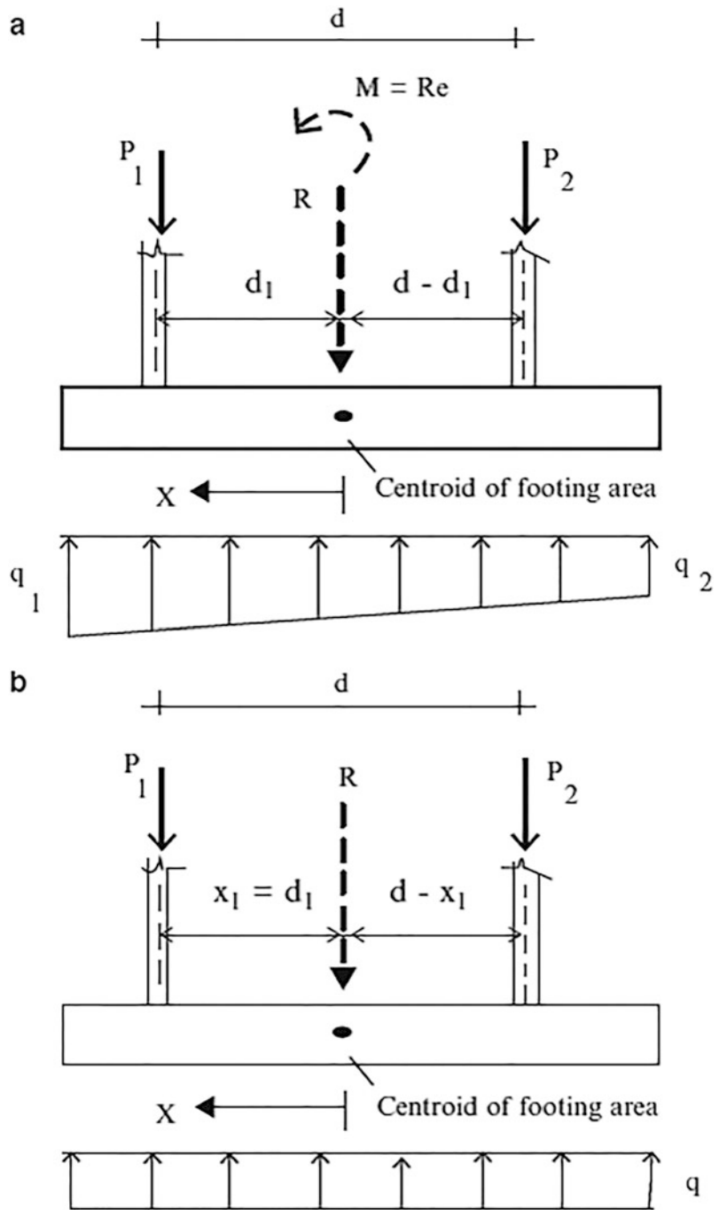
Fig. 7.14 Conditions for soil pressure distribution. (a) e > 0 . (b) e = 0
