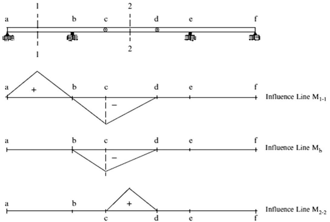
Fig. E3.28b Influence lines
