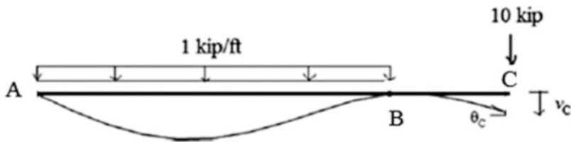
Fig. E3.23e Deflected shape
