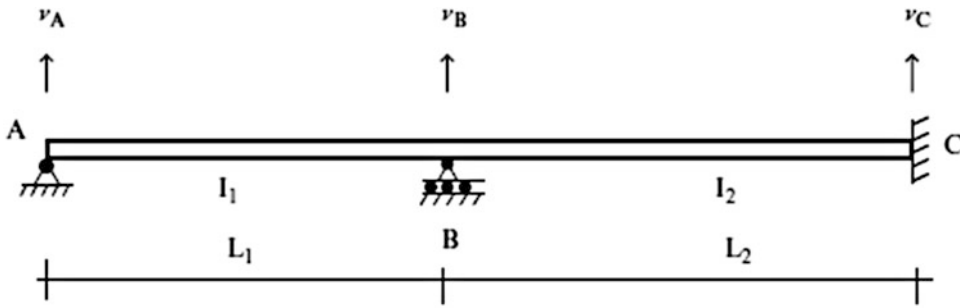
Fig. 10.11 Beam geometry and support settlements
