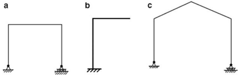
Fig. 4.4 Statically determinate support schemes for planar frames
