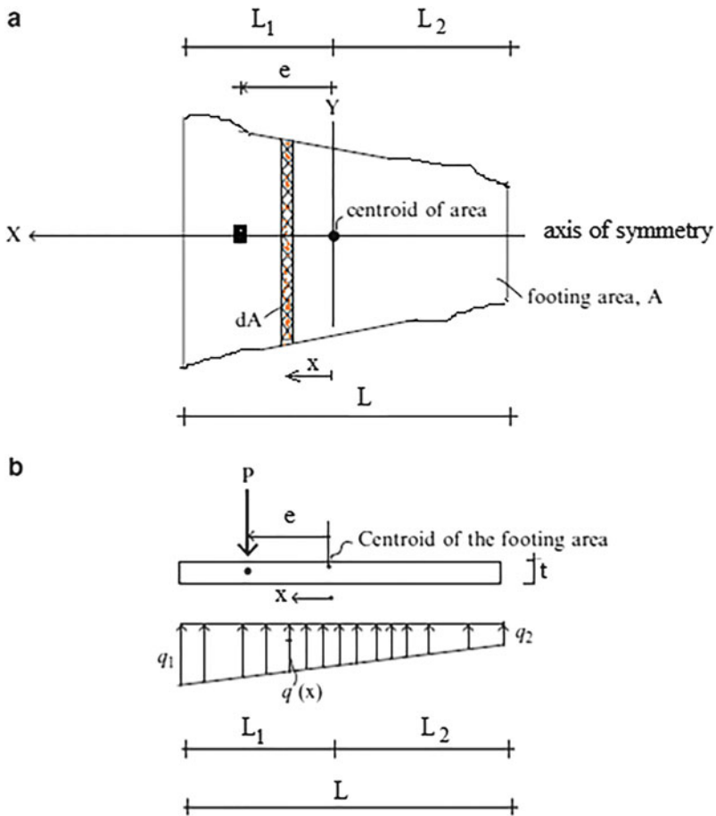
Fig. 7.7 Notation—pressure distribution—single footing. (a) Plan. (b) Elevation
