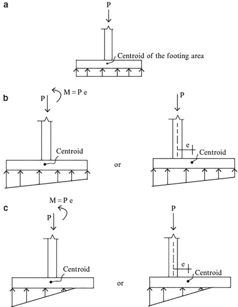
Fig. 7.6 Idealized pressure distributions. (a) Uniform. (b) Trapezoidal. (c) Triangular
