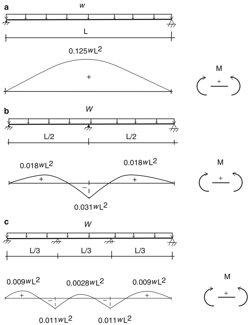
Fig. 13.10 Variation of the bending moment distribution. (a) Simply supported. (b) Two-span scheme. (c) Three-span scheme
