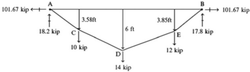
Fig. E5.1c Sag profile for v_D = 6 ft
