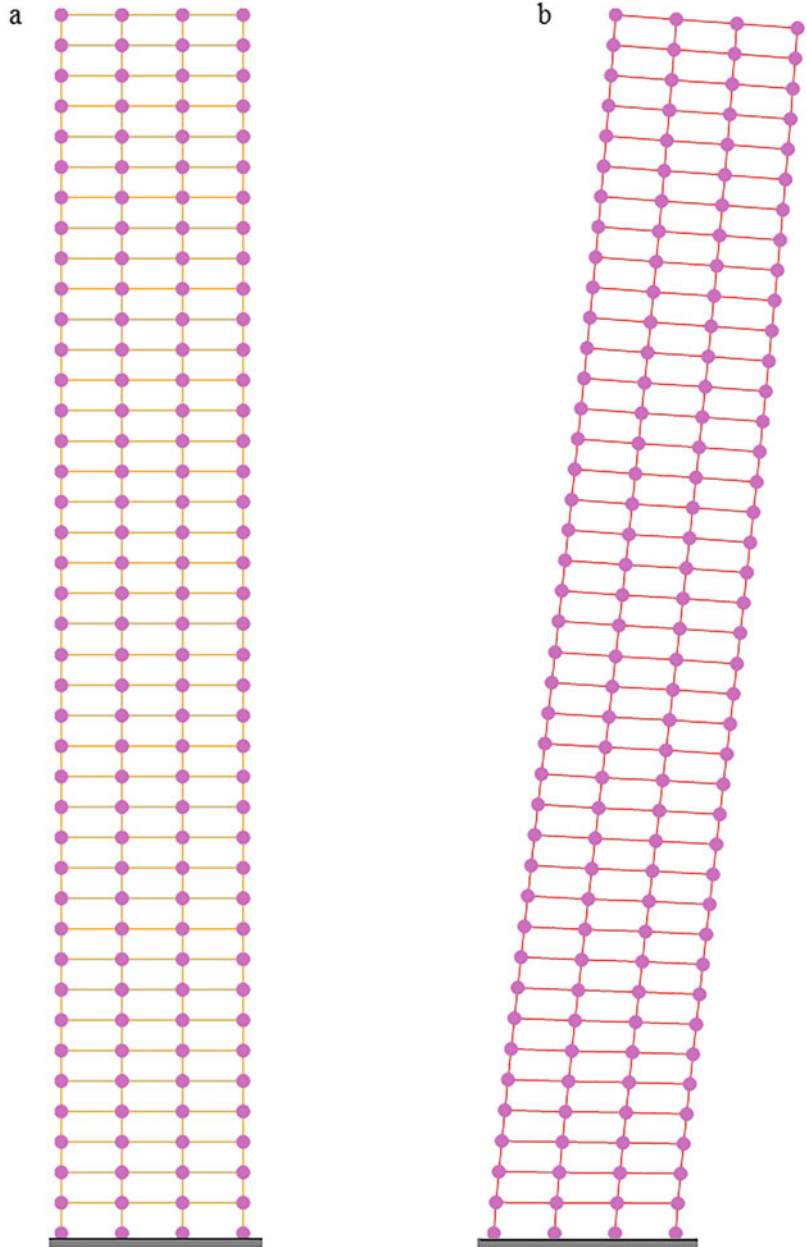
Fig. 11.17 Tall building model—lateral deflections
