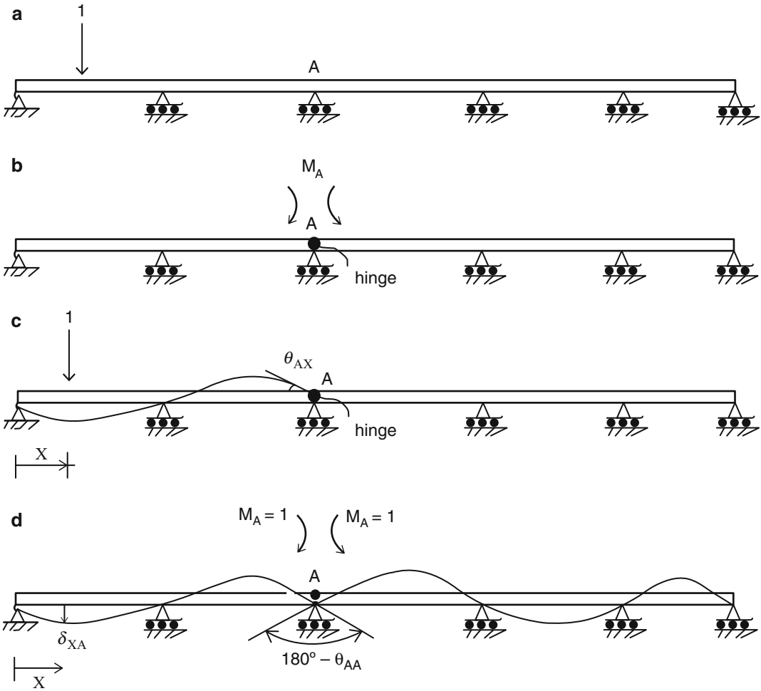
Fig. 13.2 Application of Müller-Breslau principle (a) Example structure. (b) Negative moment. (c) Deflection due to load. (d) Deflection due to moment
