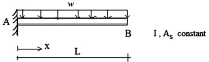
Fig. 3.33 Cantilever beam
