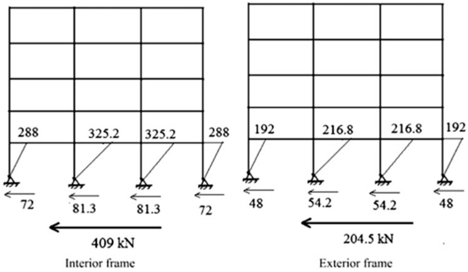
Fig. E14.16h Maximum column moments—flexible floors
