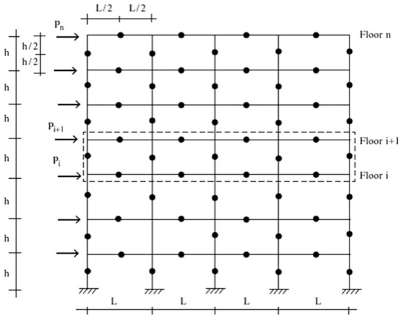
Fig. 11.8 Low-rise, frame
