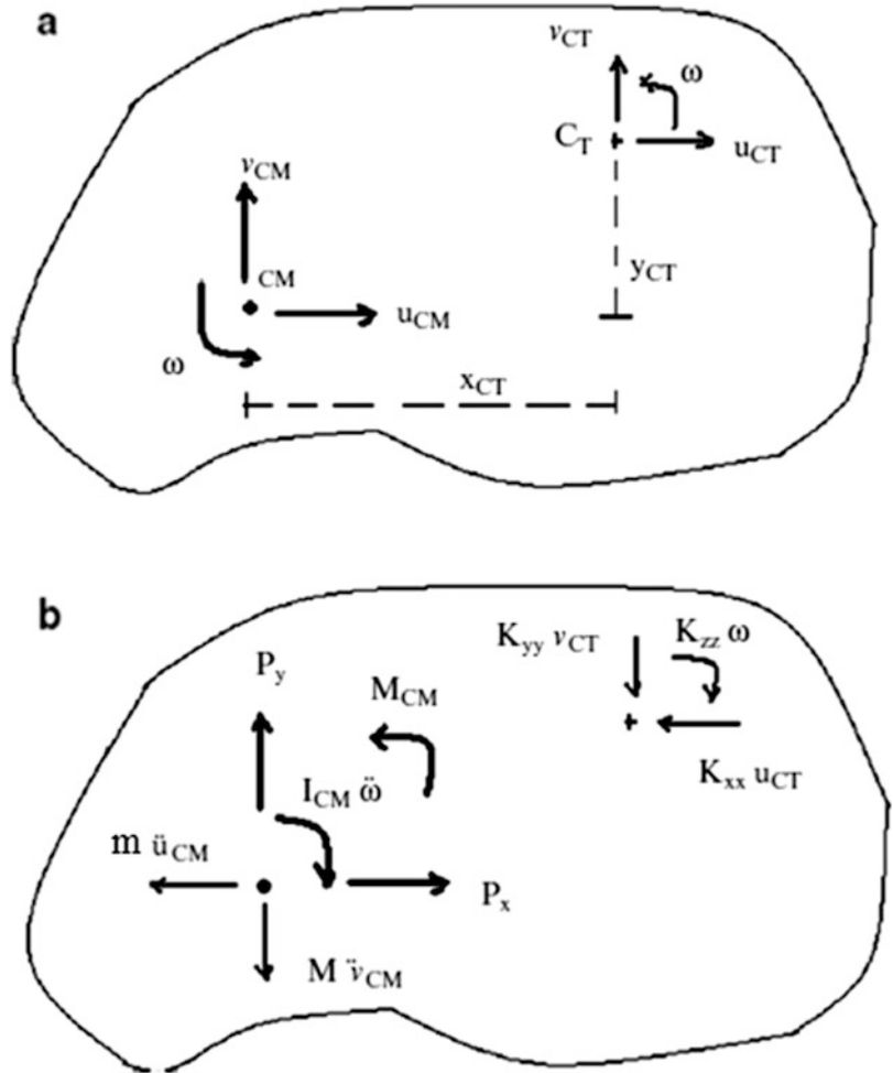
Fig. 14.18 Forces acting at the center of mass (a) Displacements, (b) Forces
