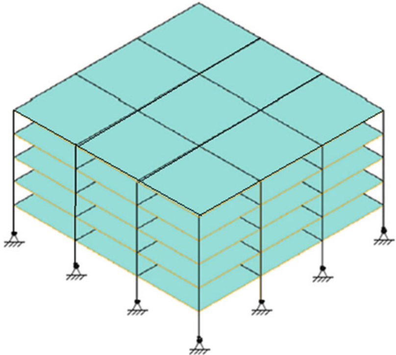
Fig. 4.36 A typical 3-D system of plane frames
