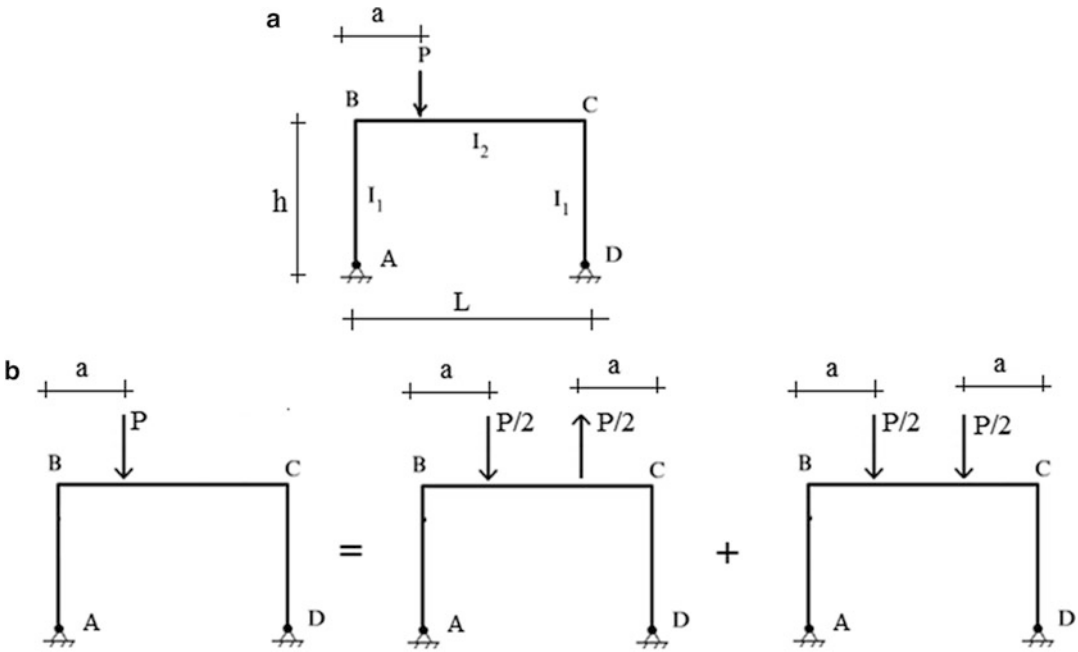
Fig. 9.40 (a) Two-hinged frame under gravity loading. (b) Decomposition of loading into symmetrical and anti-symmetrical components
