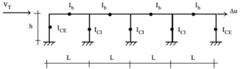
Fig. 11.11 Transverse shear model for bottom story—fixed support
