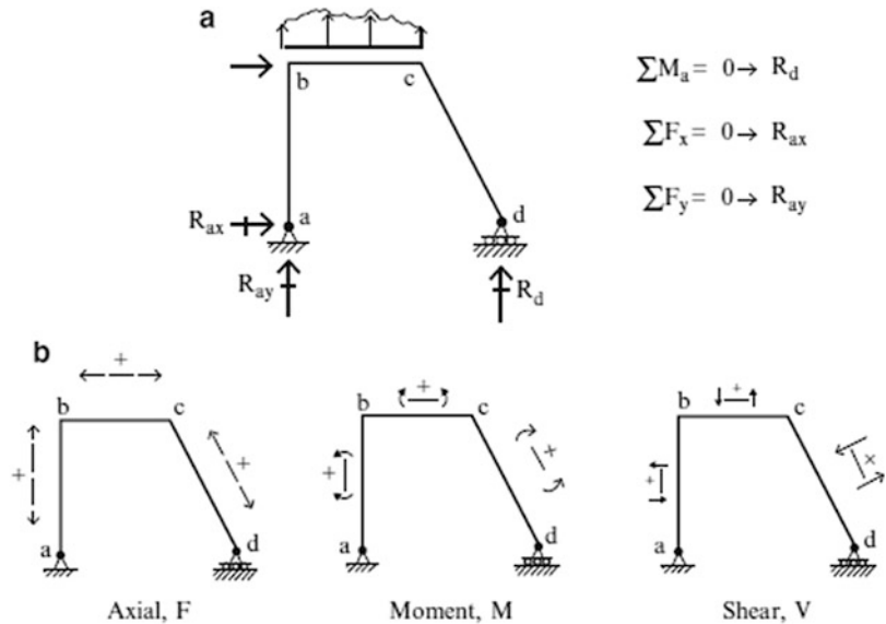
Fig. 4.10 (a) Typical frame. (b) Sign convention for the bending moment, transverse shear, and axial force
