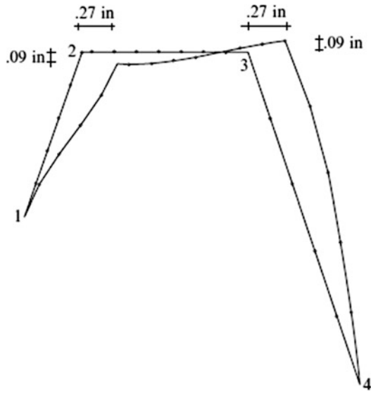
Fig. E10.19d Deflection Profile— I = 400 \text{ in.}^4
