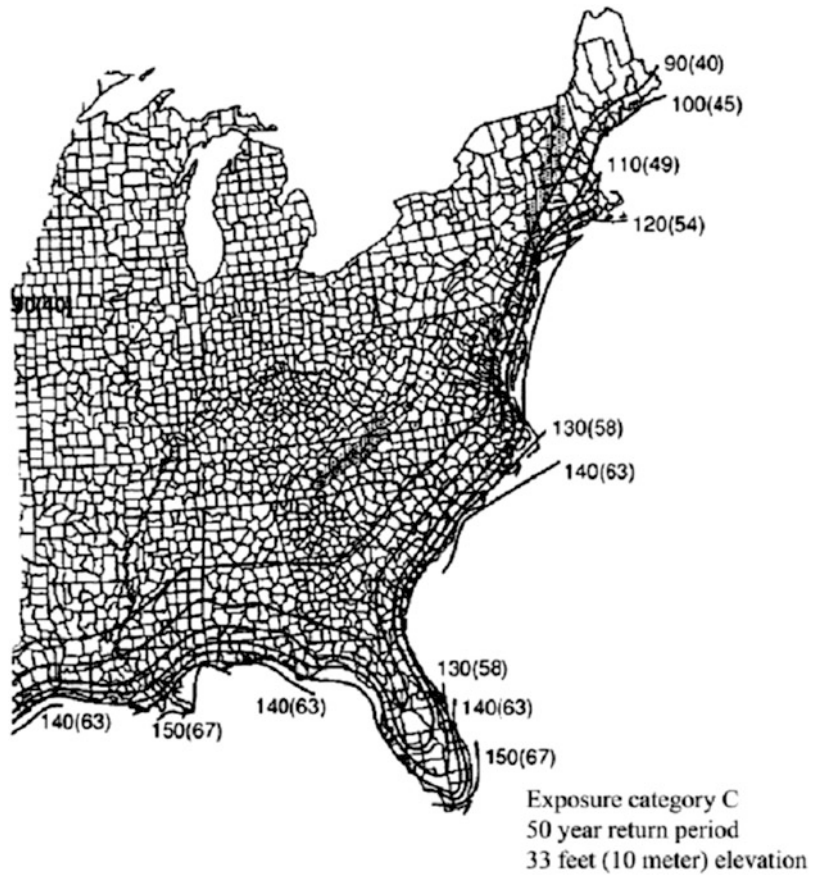
Fig. 1.13 Basic wind speed miles per hour (meter per second) for the East coast of the USA
