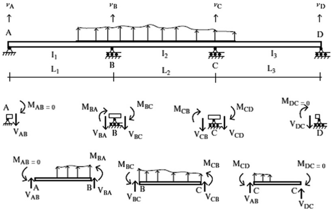
Fig. 10.12 Three-span beam
