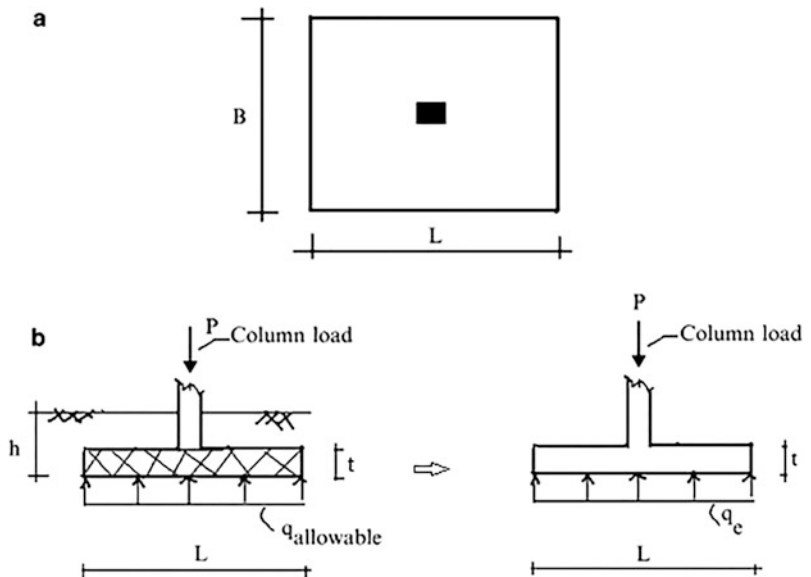
Fig. 7.10 Notation-effective soil pressure ( q_e ). (a) Plan. (b) Elevation
