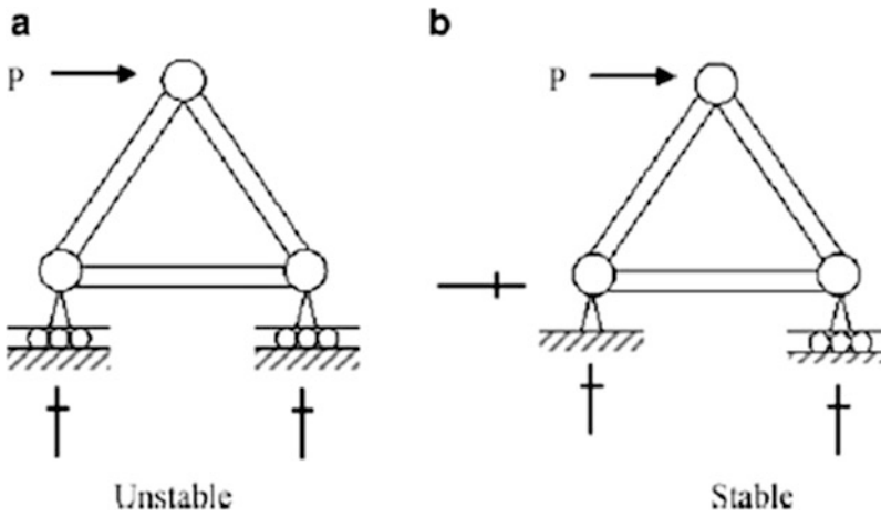
Fig. 1.4 Examples of unstable and stable support conditions—planar structure
