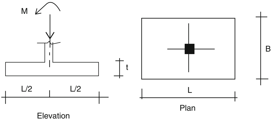
Fig. E7.2a Geometry and loading
