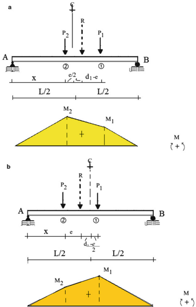
Fig. 3.53 Critical location of loading for maximum bending moments. (a) x|_{M_{2max}} , (b) x|_{M_{1max}}
