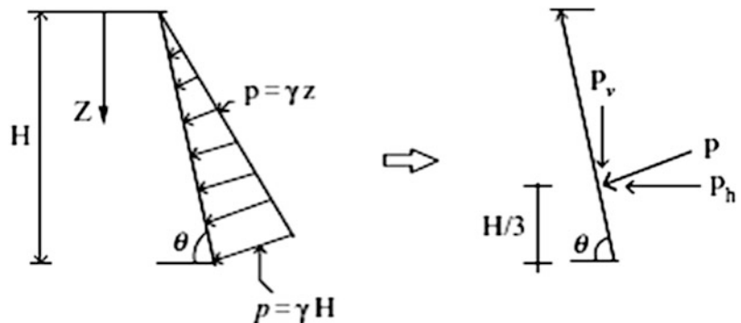
Fig. 8.6 Hydrostatic forces on an inclined surface
