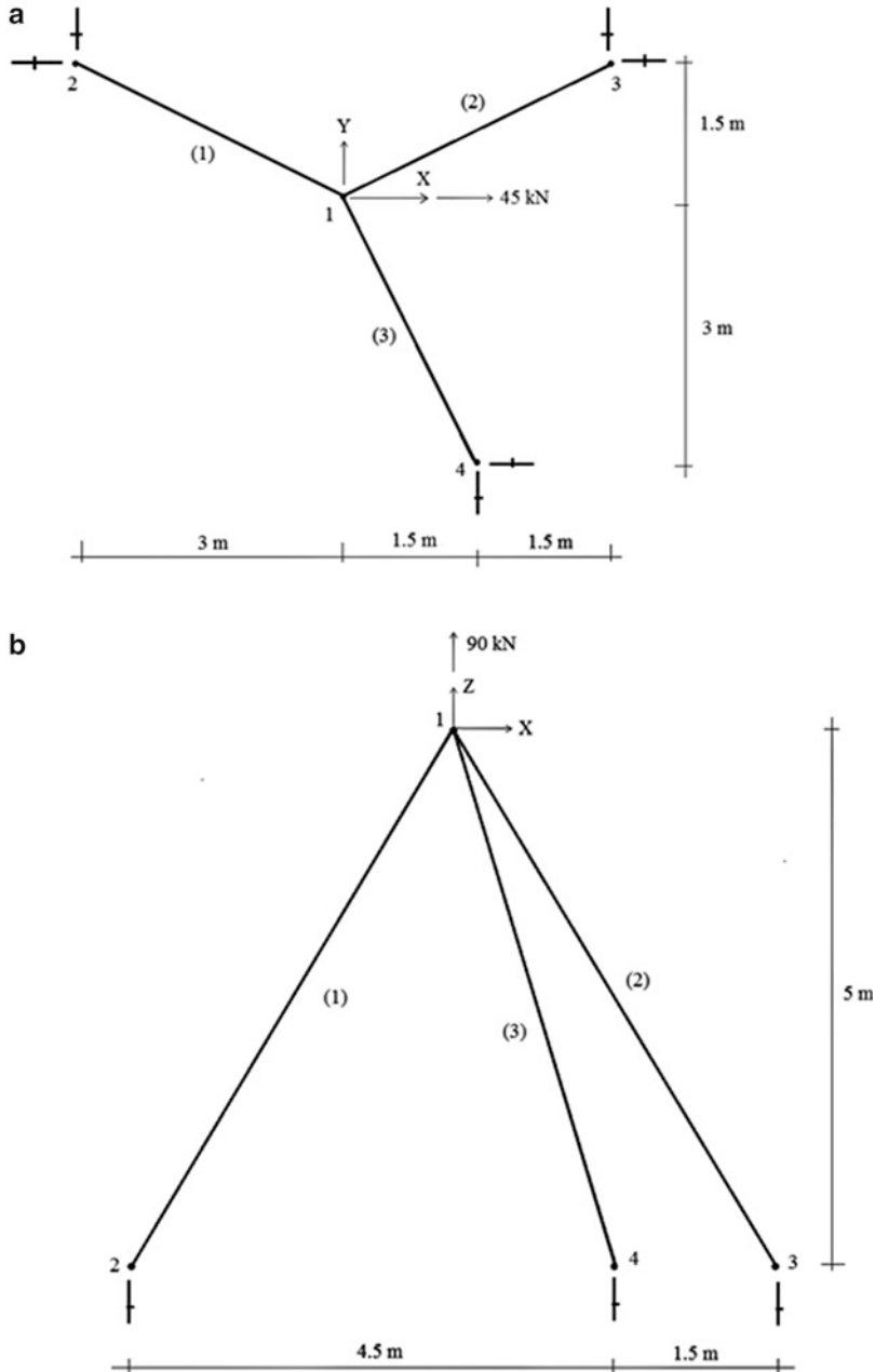
Fig. E12.13 Space truss geometry and supports. (a) x - y plan view. (b) x - z plan view
