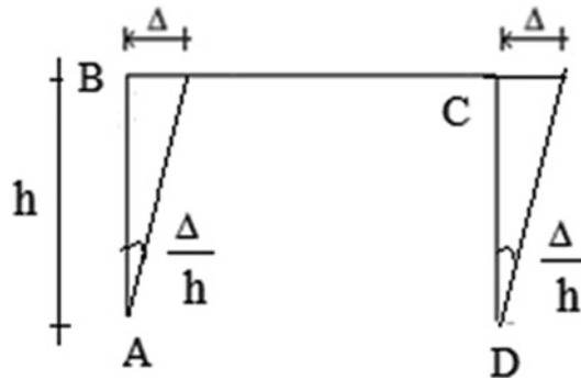
Fig. E10.17d Case II—sideway introduced
