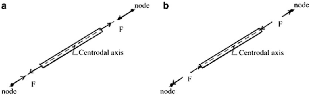
Fig. 2.14 Free body diagram of a truss member and its associated nodes. (a) Tension. (b) Compression
