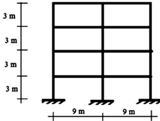
Elevation—Section A-A
