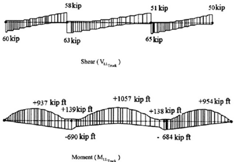
Fig. 13.25 Truck loading envelopes
