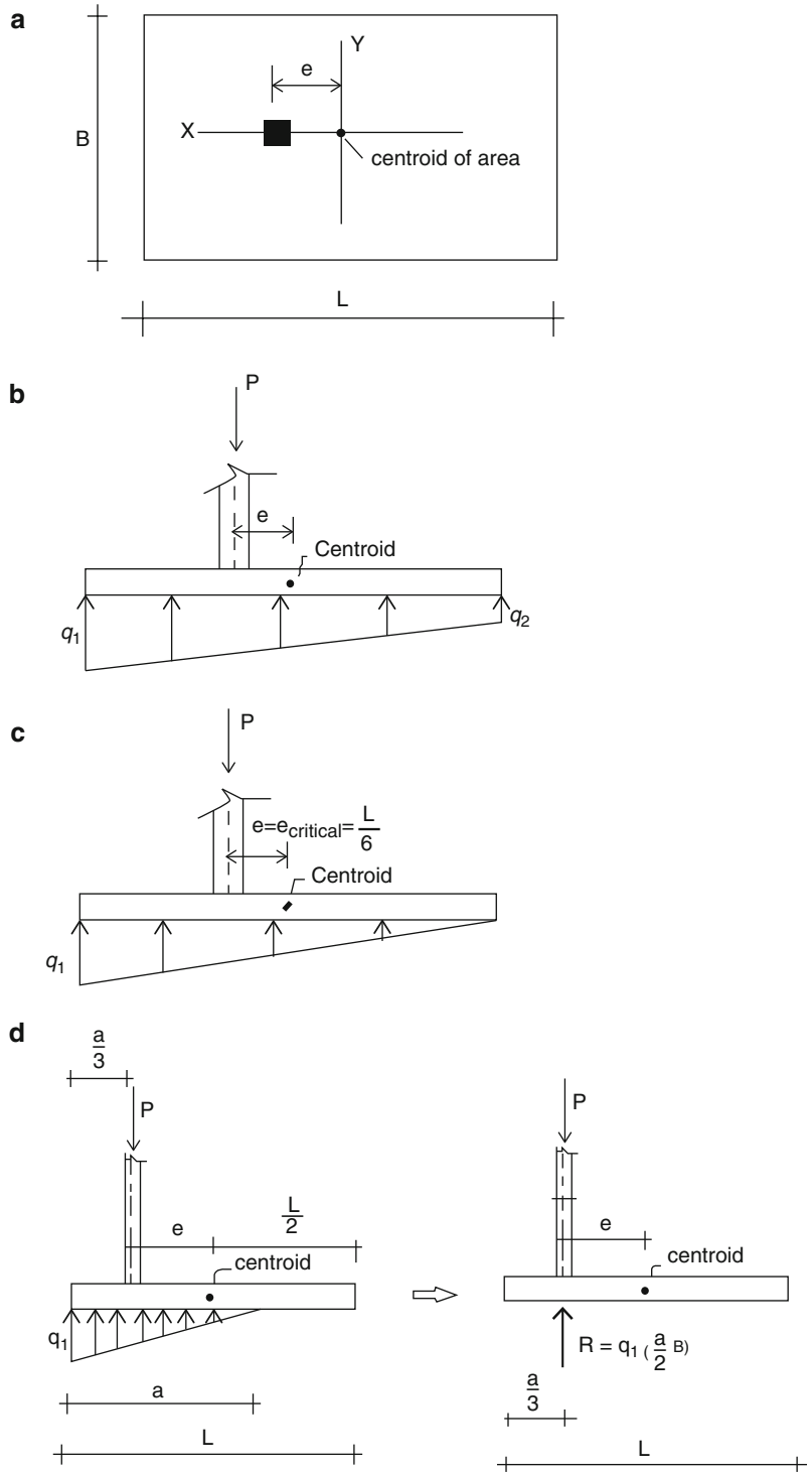
Fig. 7.9 (a) Plan—rectangular area. (b) Elevation e < e_{critical} . (c) Elevation e = e_{critical} . (d) Pressure distribution for e > e_{critical}
