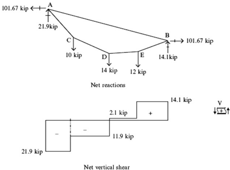
Fig. E5.2d Vertical shear
