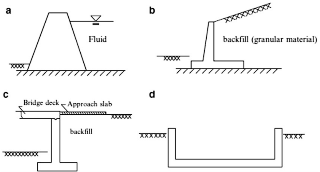
Fig. 8.1 Vertical retaining wall structures. (a) Gravity dam. (b) Cantilever retaining wall. (c) Bridge abutment. (d) Underground basement
