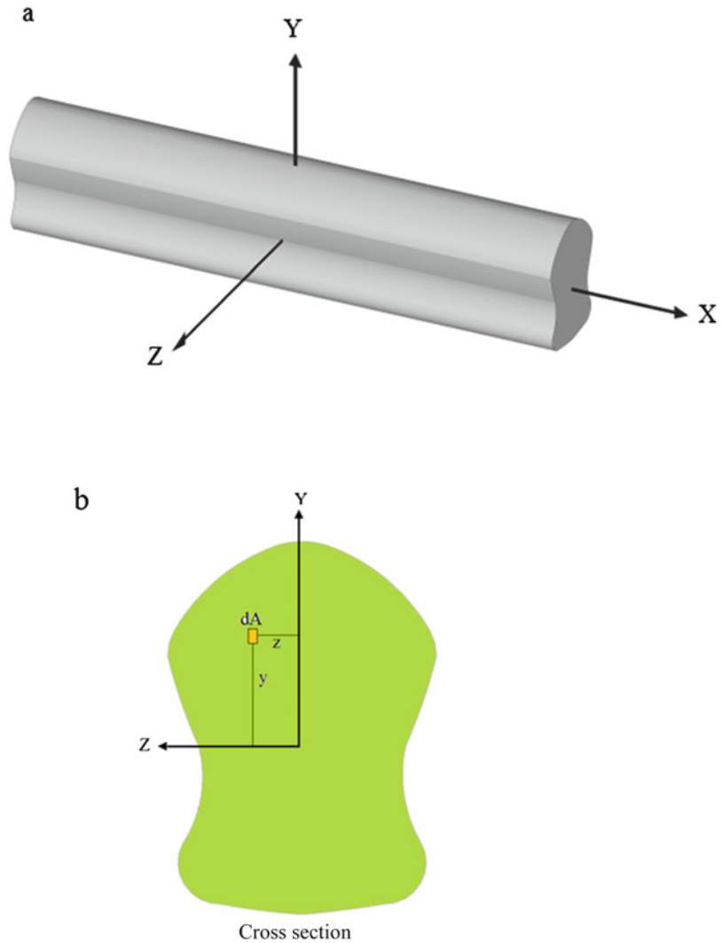
Fig. 3.2 Notations for prismatic beam—symmetrical cross-section
