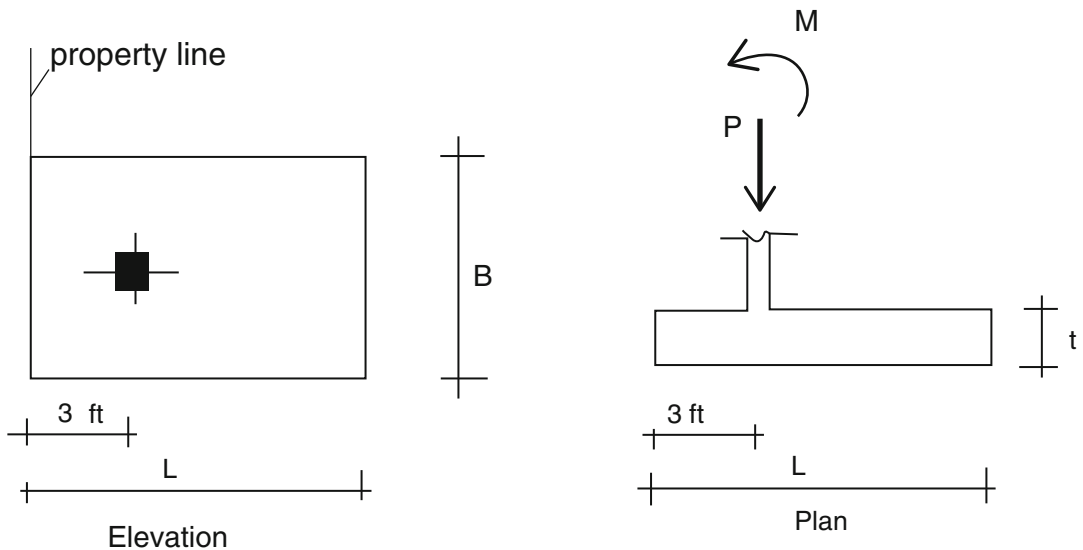
Fig. E7.2d Geometry and loading
