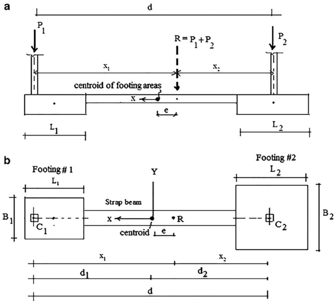
Fig. 7.17 Notation and pressure distribution for strap footing. (a) Elevation. (b) Plan
