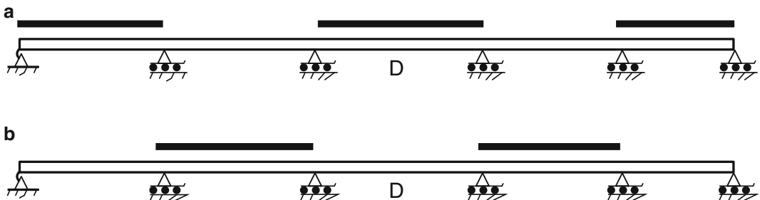
Fig. 13.5 Loading zones for moment at D. (a) Positive value. (b) Negative value
