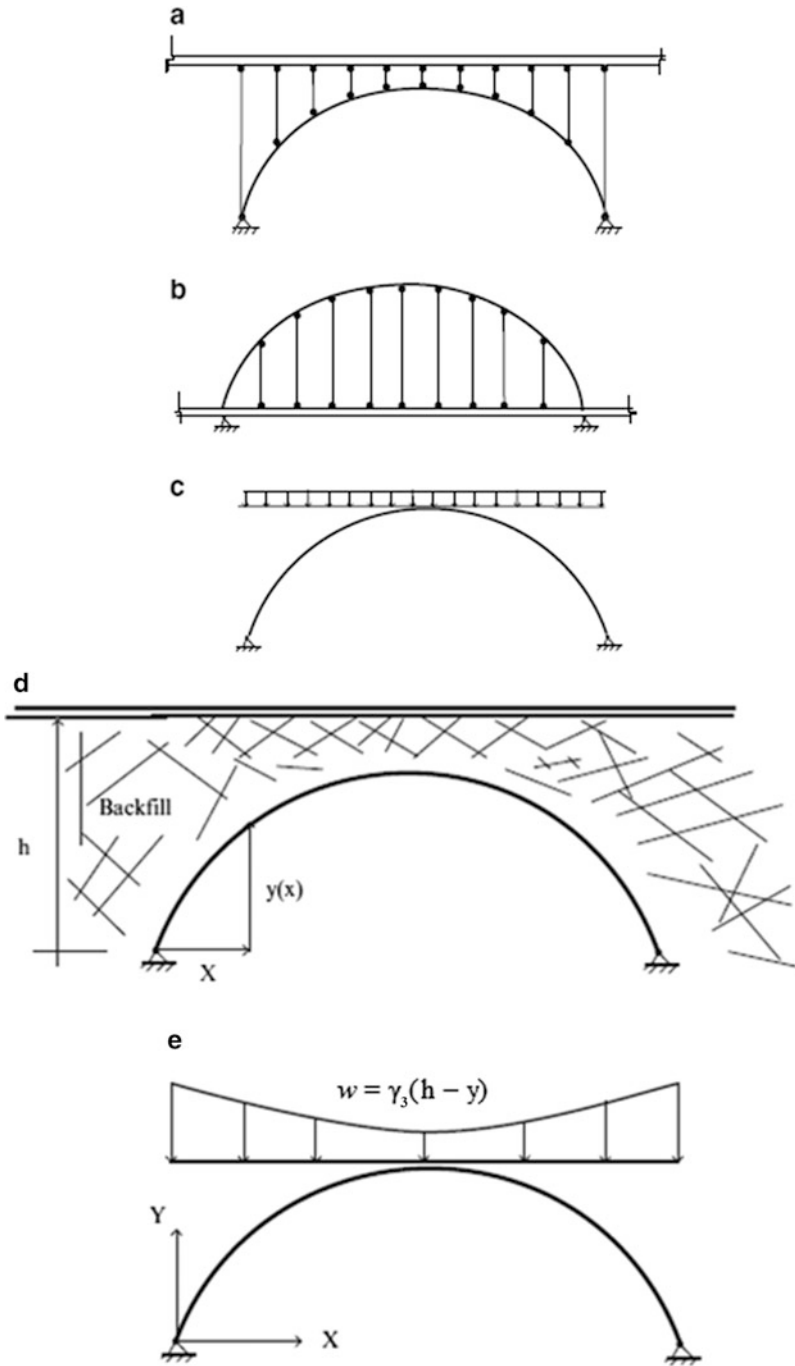
Fig. 6.11 Different roadway arrangements—idealized loading. (a) Roadway above the arch. (b) Roadway below the arch. (c) Idealized uniform dead loading. (d) Soil backfill above the arch. (e) Idealized soil loading
