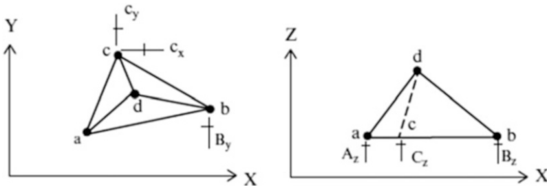
Fig. E2.21h Alternative restraint scheme #3
