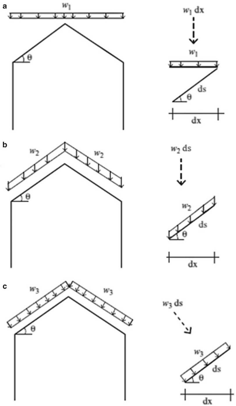
Fig. 4.17 Loading on an inclined member. (a) Vertical load per horizontal projection. (b) Vertical load per length. (c) Normal load per length
