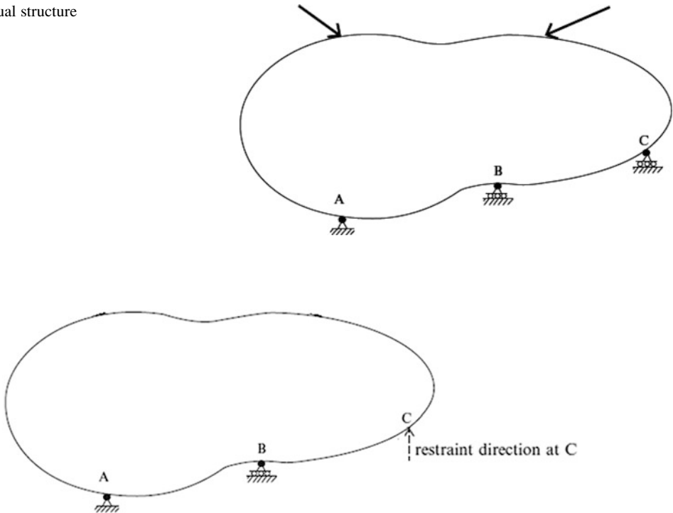
Fig. 9.2 Primary structure
