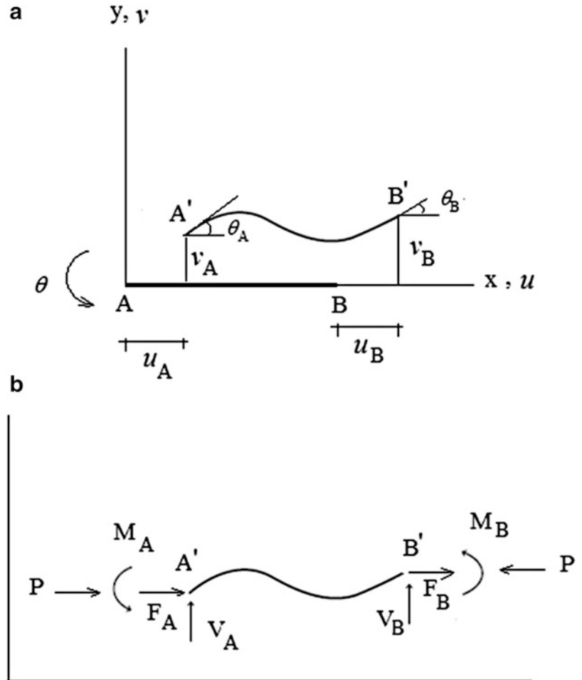
Fig. 10.34 Notation for nonlinear case. (a) Displacements. (b) End actions
