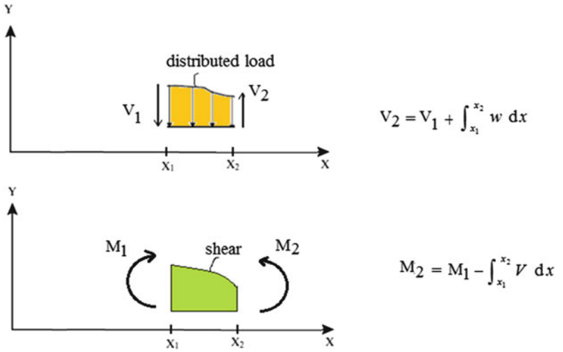
Fig. 3.16 Interpretation of shear and moment in terms of segmental loadings
