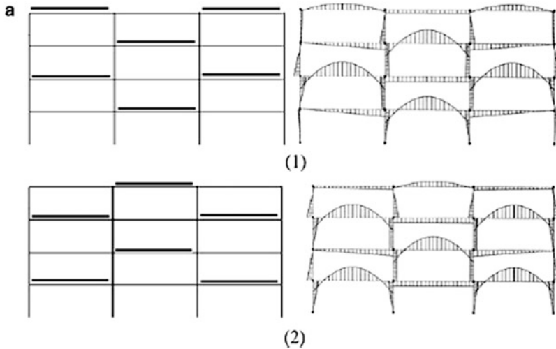
Fig. 15.18 (a) Positive live load (LL) moment patterns (1)–(2). (b) Negative live load (LL) moment patterns (3)–(10). (c) Live load patterns for axial force in column (11)–(12)
