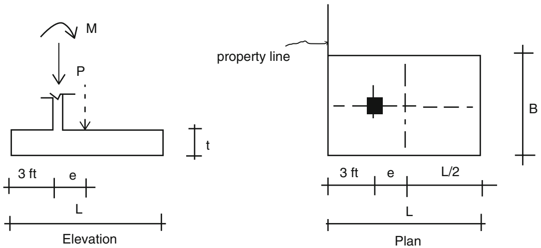
Fig. E7.2b Geometry and loading
