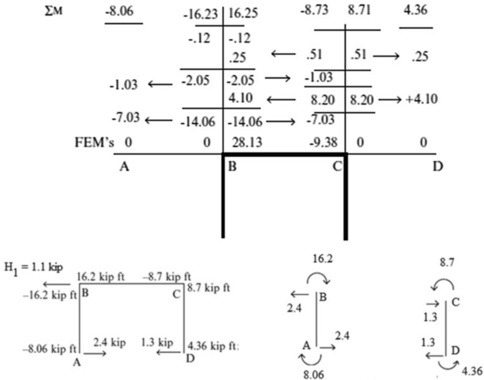
Fig. E10.17c Case I—end moments and column shear
