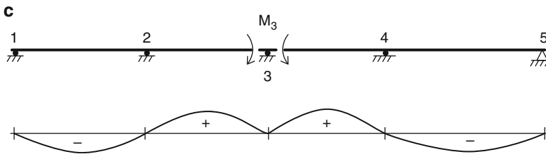
Fig. E13.1c Influence line for M_3
