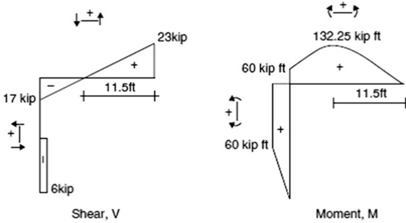
Fig. E4.3d Shear and moment diagrams
