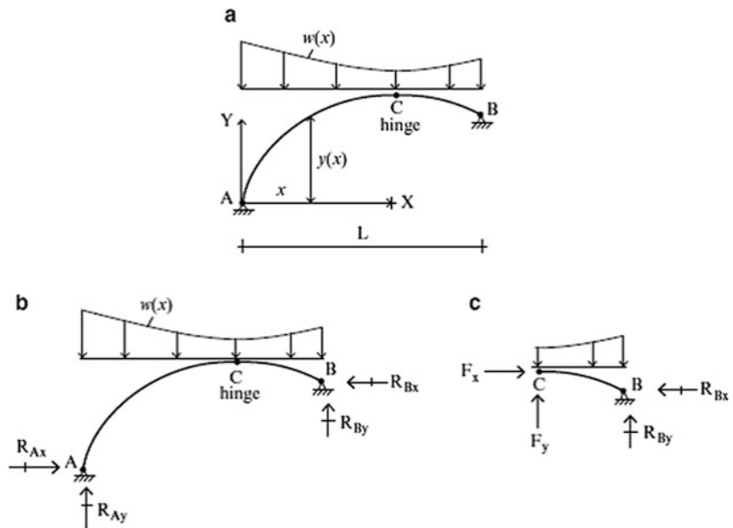
Fig. 6.19 Geometry and reactions—three-hinged arch. (a) Geometry. (b) Reactions. (c) Right segment
