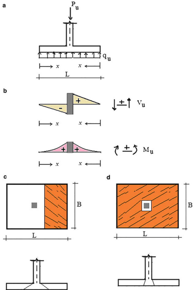
Fig. 7.11 Footing dimensioning process. (a) Factored soil pressure. (b) Shear and moment diagrams. (c) One way shear. (d) Punching shear
