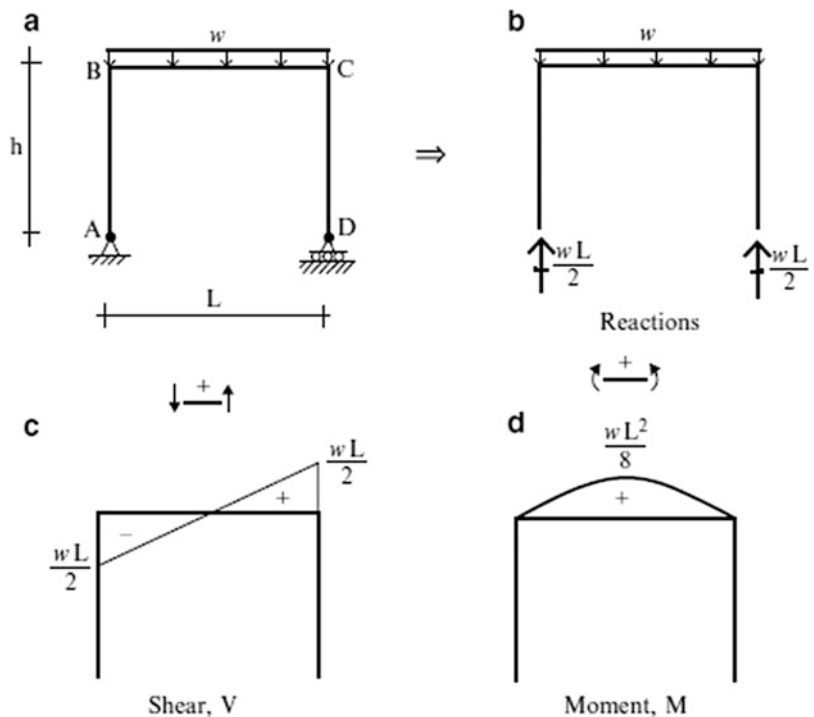
Fig. 4.11 Statically determinate portal frame under gravity loading. (a) Geometry and loading. (b) Reactions. (c) Shear diagram. (d) Moment diagram
