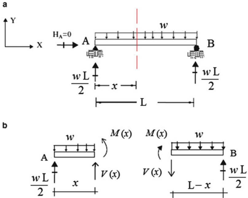
Fig. 3.12 Internal shear and moment. (a) beam. (b) Segmented beam
