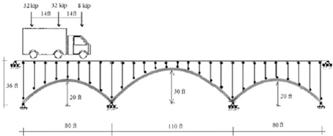
Fig. 13.31 Idealized model—three-span arch
