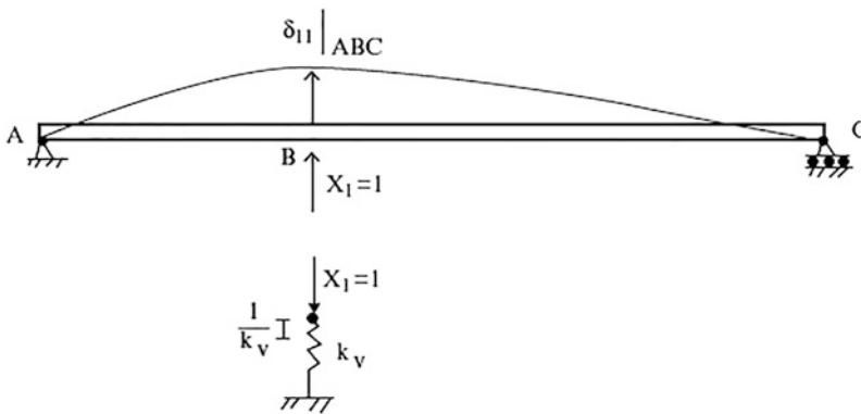
Fig. E9.4b Deflected shape due to X_1 = 1
