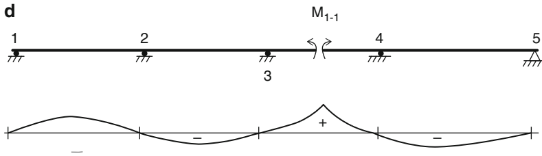
Fig. E13.1d Influence line for M_{1-1}
