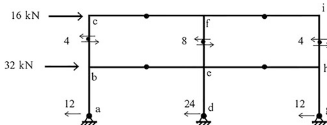
Fig. E11.1b Shear distribution for the columns (kN)
