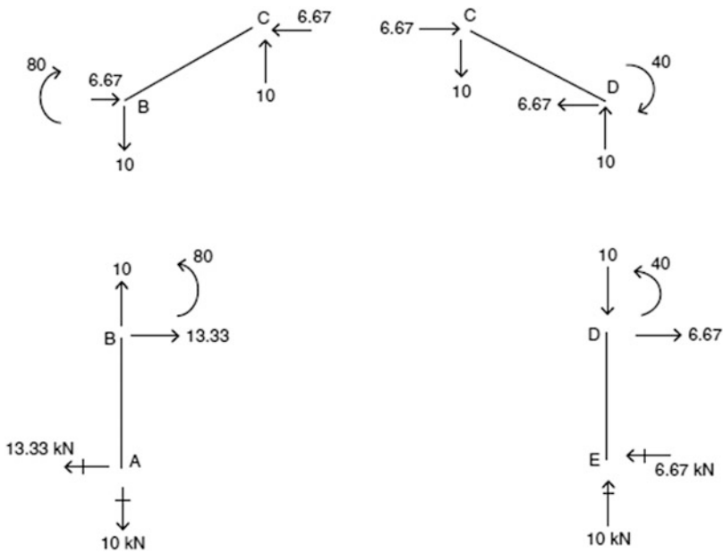
Fig. E4.8c End forces
