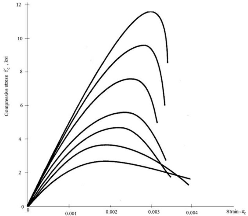
Fig. 16.7 Compressive stress–strain curves for concrete
