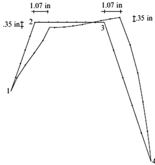
Fig. E10.19b Deflection profile— I = 100 \text{ in.}^4
