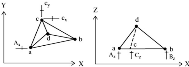
Fig. E2.21g Alternative restraint scheme #2
