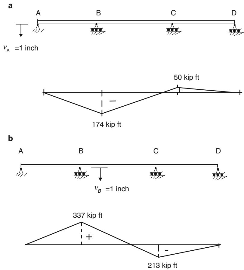
Fig. 13.26 Moment due to support settlements ( E = 29,000 ksi and I = 48,110 in. 4 ). (a) Settlement at A. (b) Settlement at B
