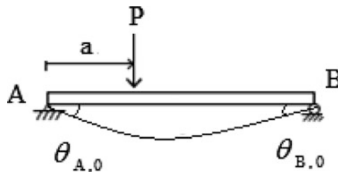
Fig. E9.7c Deformation of primary structure due to external loading
