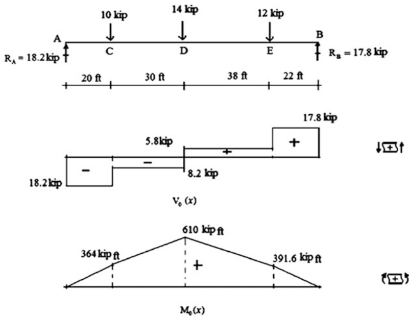
Fig. E5.1b Simply supported beam results
