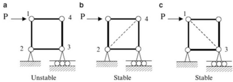
Fig. 1.5 Stabilizing an initially unstable planar structure
