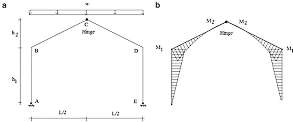
Fig. 9.55 Three-hinge solution. (a) Loading. (b) Bending moment distribution
