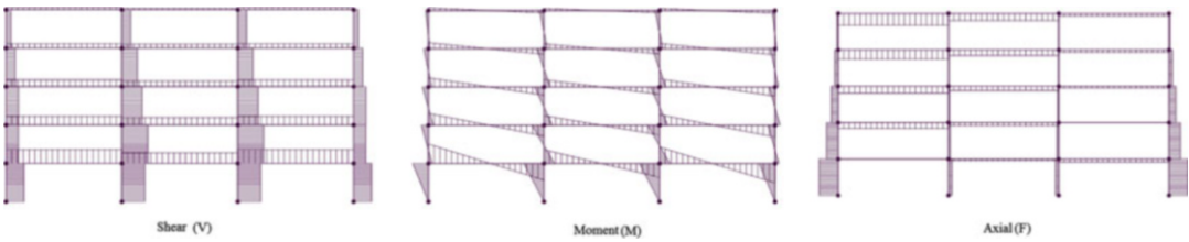
Fig. E15.2f Shear, moment, axial force diagrams—earthquake loading
