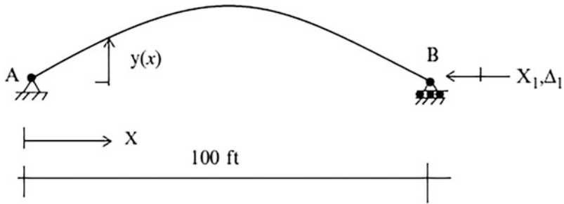
Fig. E9.13b Primary structure—redundant reaction
