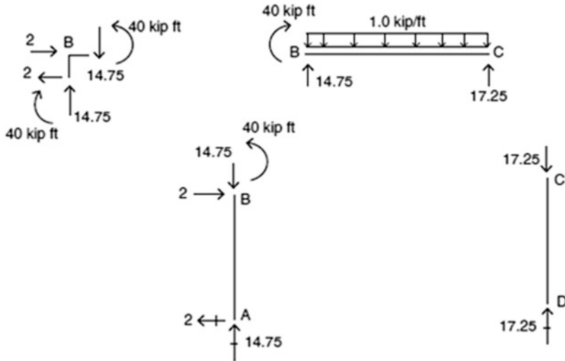
Fig. E4.4c End actions
