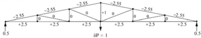
Fig. E2.17c Virtual forces \delta F_v
