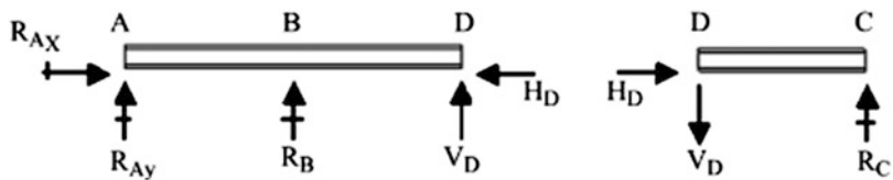
Fig. 3.9 Free body diagram for beam with moment release
