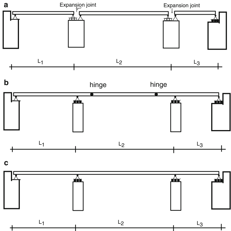
Fig. 13.7 Multi-span bridge schemes (a) Simple spans. (b) Cantilever spans. (c) Continuous spans
