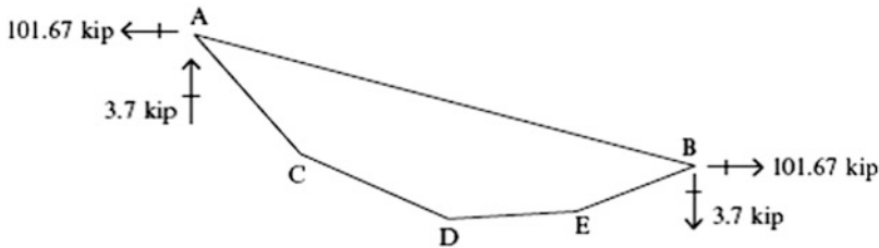
Fig. E5.2c Vertical reactions due to H
