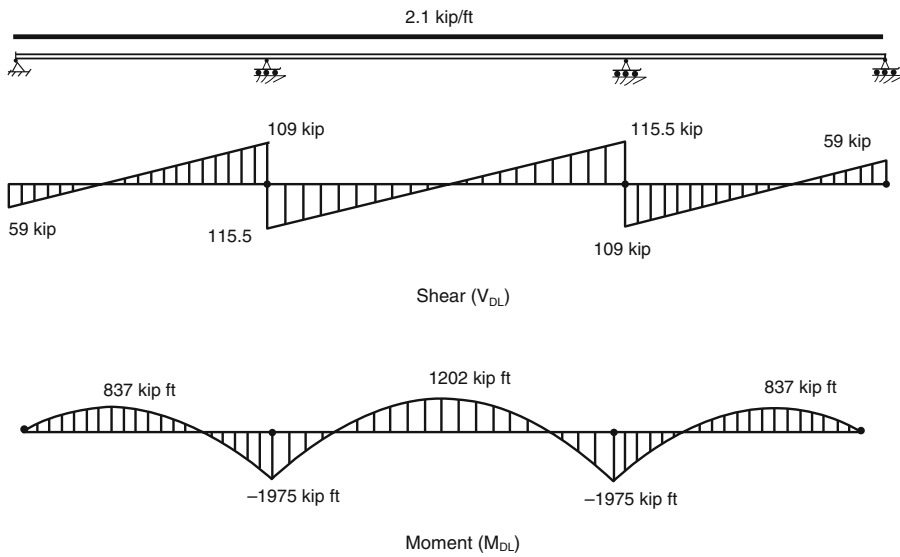
Fig. 13.23 Dead load shear and moment distributions
