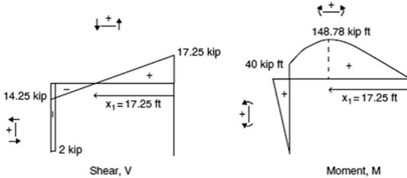
Fig. E4.4d Shear and moment diagrams
