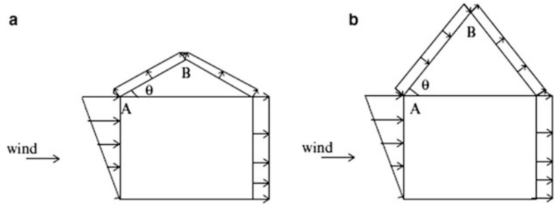
Fig. 1.12 Wind pressure profiles for a gable roof. (a) \theta < 45^\circ . (b) \theta > 45^\circ
