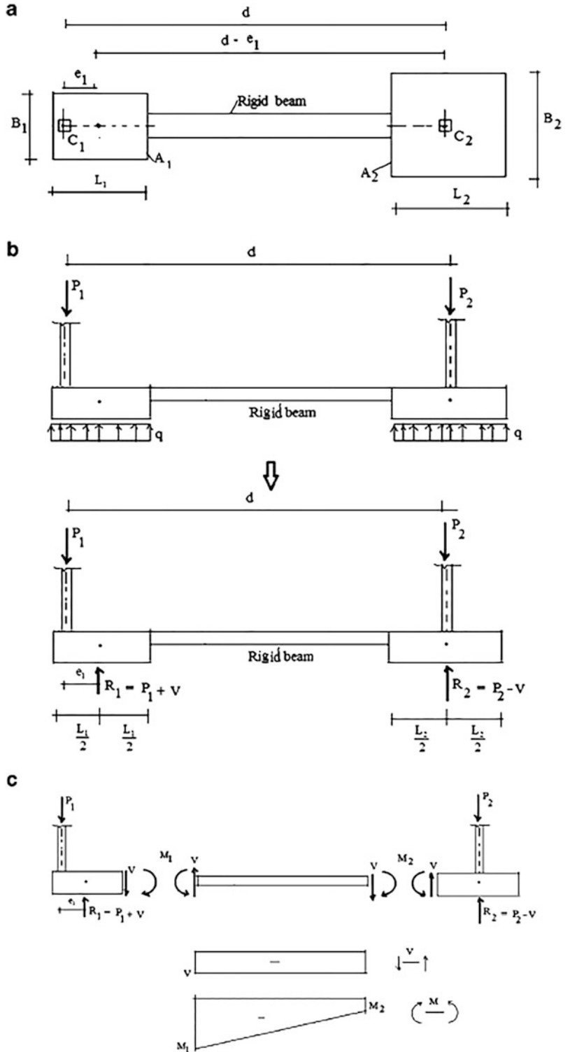
Fig. 7.19 Approximate strap footing analysis. (a) Plan (b) Elevation (c) Components of footing
