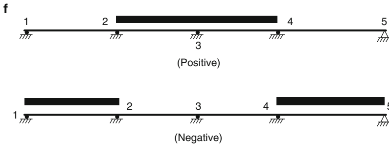
Fig. E13.1f Loading patterns for absolute maximum R_3
