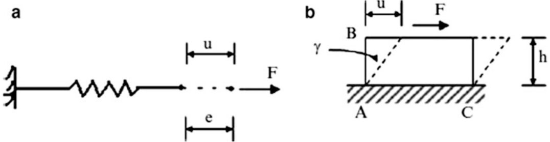
Fig. 1.28 Deformation modes. (a) Extension. (b) Shear
