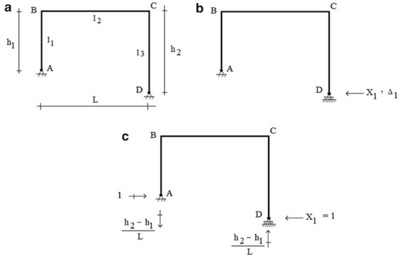
Fig. 9.33 Portal Frame. (a) Geometry. (b) Redundant. (c) Reactions due to X_1 = 1
