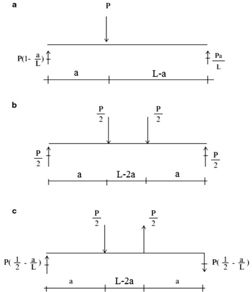
Fig. 3.43 Representation of an arbitrary loading by superposition. (a) Single concentrated load. (b) Set of symmetrical loads. (c) Set of anti-symmetrical loads
