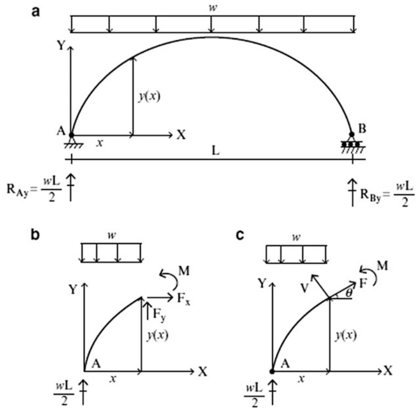
Fig. 6.15 Curved member—uniform vertical loading. (a) Reactions. (b) Internal forces—Cartesian frame. (c) Internal forces—local frame
