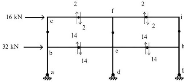
Fig. E11.1f Shear distribution for the beams (kN)
