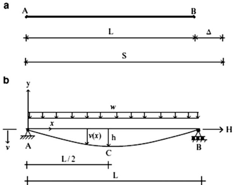
Fig. 5.17 Cable geometry. (a) Initial unloaded. (b) Loaded shape
