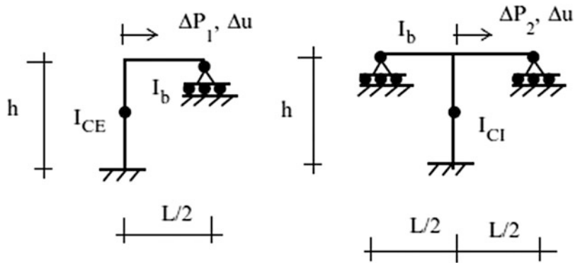
Fig. 11.12 Typical sub-elements for base story—fixed support. (a) Exterior. (b) Interior
