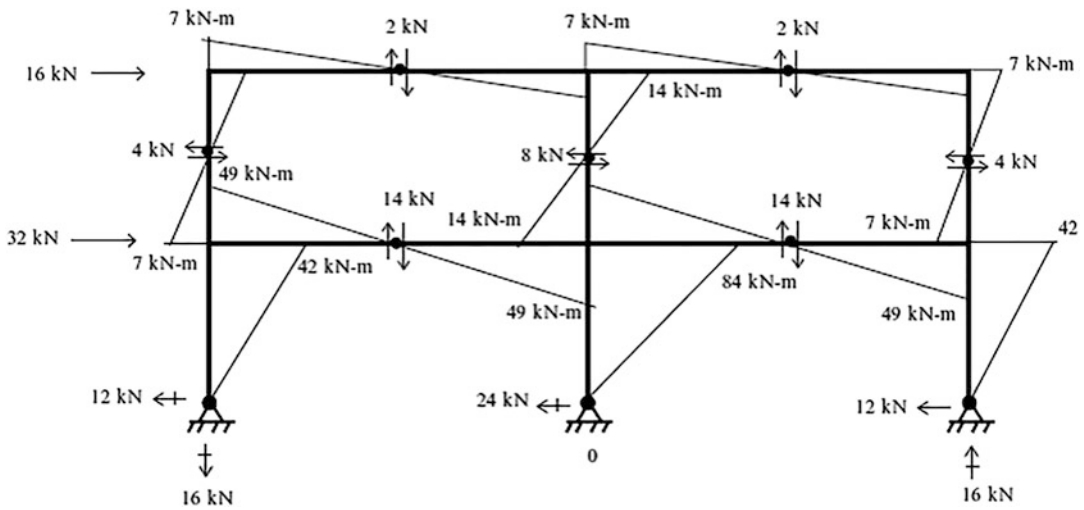
Fig. E11.1h Reactions, shear forces, and moment distribution
