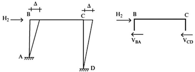
Fig. 10.24 Sideway introduced—case II
