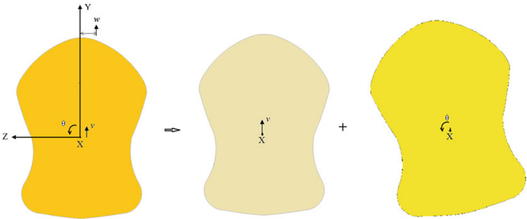
Fig. 3.4 Combined bending and torsion
