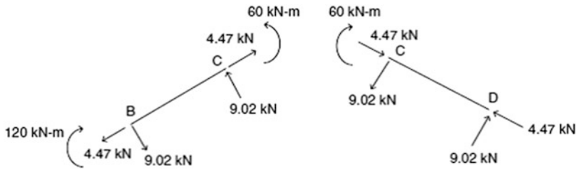
Fig. E4.7d End forces in local member frame
