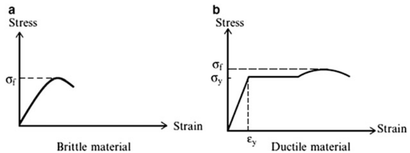
Fig. 1.6 Stress–strain behavior of brittle and ductile materials
