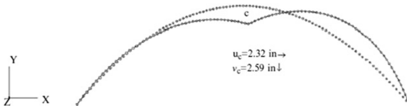
Fig. E6.8e Deflection profile
