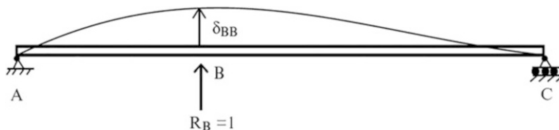
Fig. E9.2c Deflected shape due to unit value of R_B
