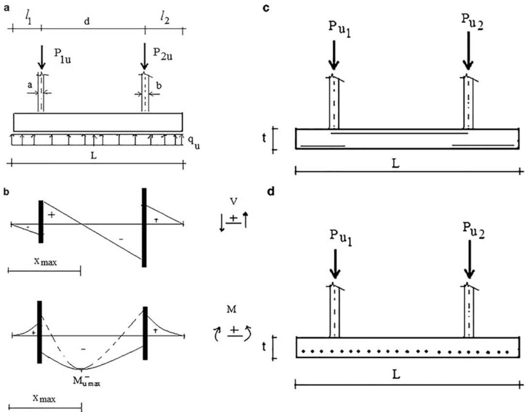
Fig. 7.15 (a) Rectangular footing with uniform ultimate soil pressure e_u = 0 . (b) Shear and Moment diagrams e_u = 0 . (c) Steel reinforcing pattern for longitudinal bending. (d) Steel reinforcing pattern for transverse bending
