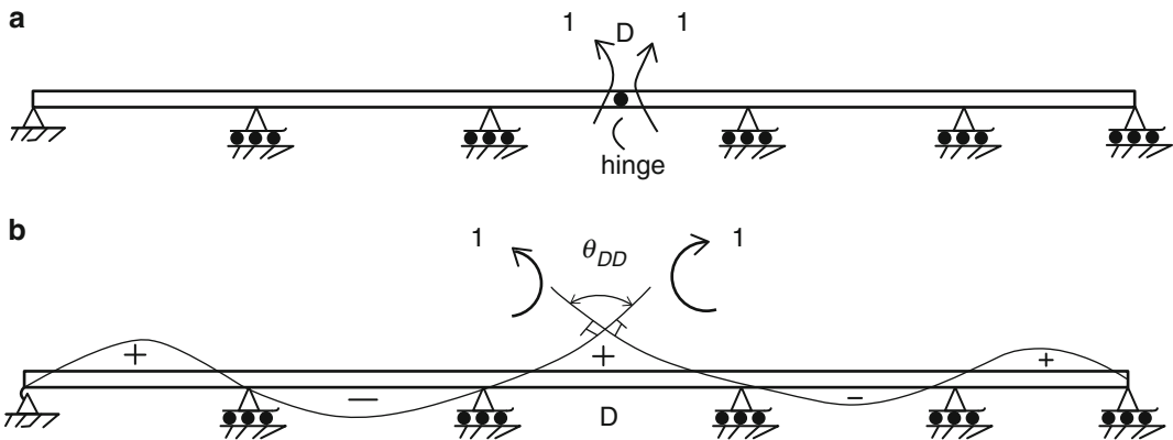
Fig. 13.4 Modified structure and deflected shape for positive moment at D
