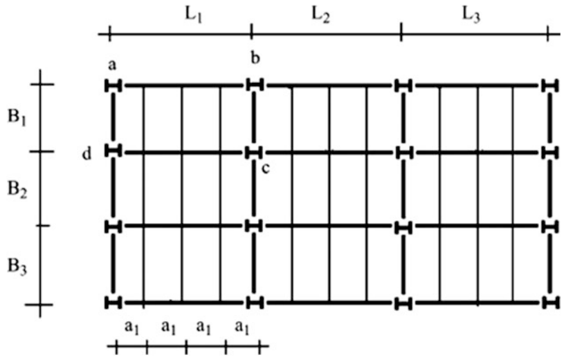
Fig. 15.6 Steel joist/beam framing scheme
