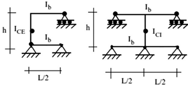
Fig. 11.10 Typical sub-elements. (a) Exterior. (b) Interior
