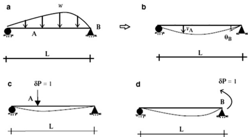
Fig. 3.28 Actual and virtual loads moments. (a) Actual load M(x) . (b) Deflected shape. (c) Virtual load \delta M_v for v_A . (d) Virtual load \delta M_\theta(x) for \theta_B
