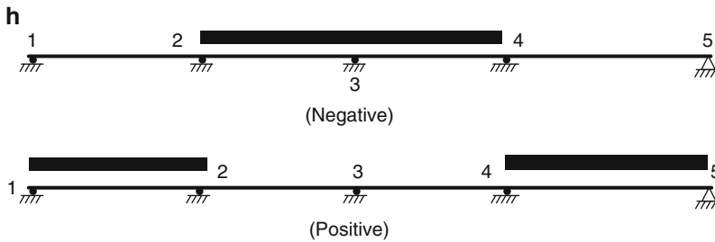
Fig. E13.1h Loading patterns for absolute maximum M_3
