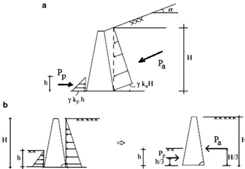
Fig. 8.10 (a) Soil pressure distribution for Rankine theory \alpha \neq 0 . (b) Soil pressure distribution for Rankine theory \alpha = 0
