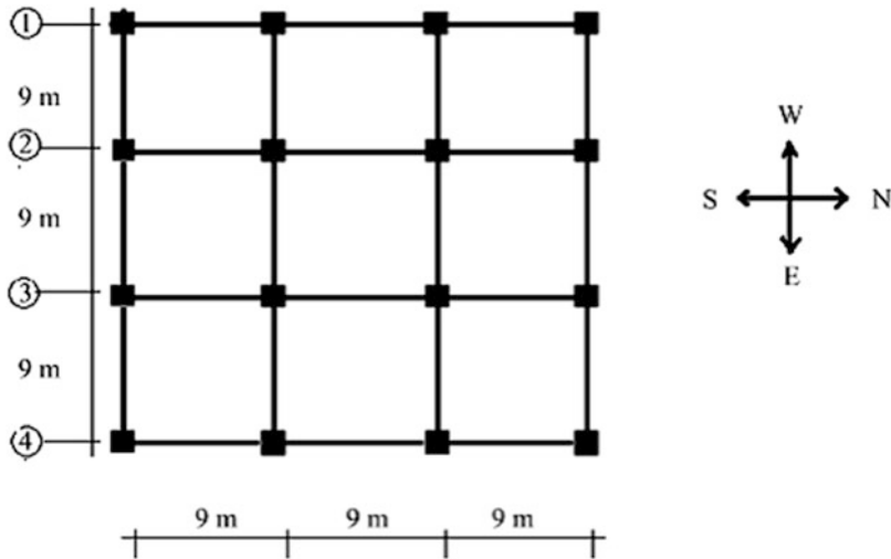
Fig. E14.16b Typical floor plan
