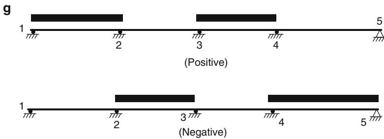
Fig. E13.1g Loading patterns for absolute maximum M_{1-1}
