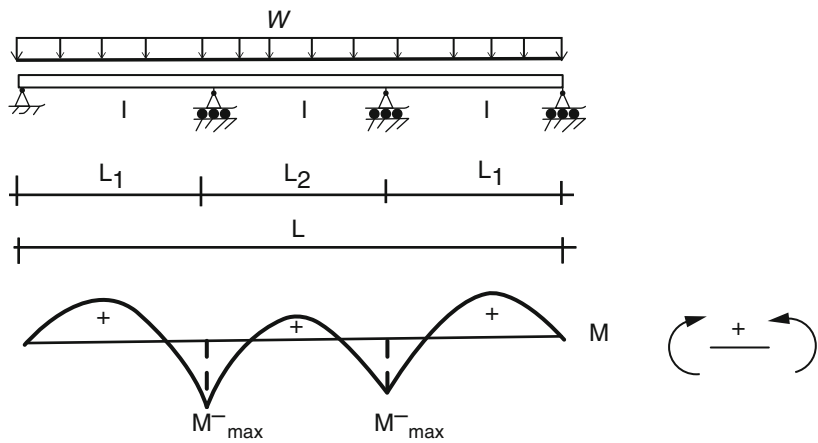
Fig. 13.11 Bending moment distribution—three-span symmetrical scheme
