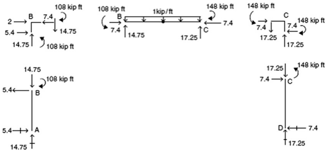
Fig. E4.5f End actions
