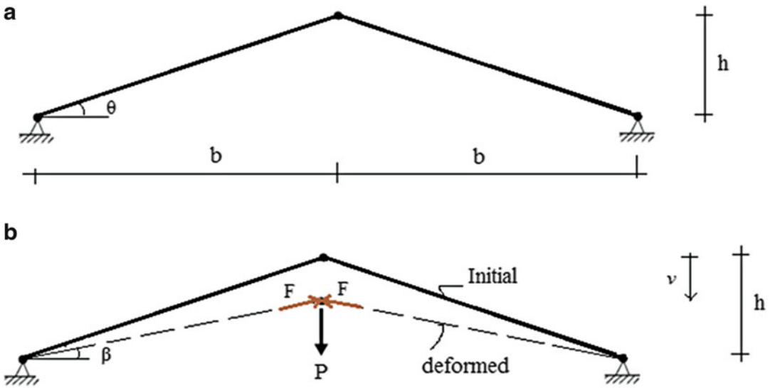
Fig. 10.28 Nonlinear truss example
