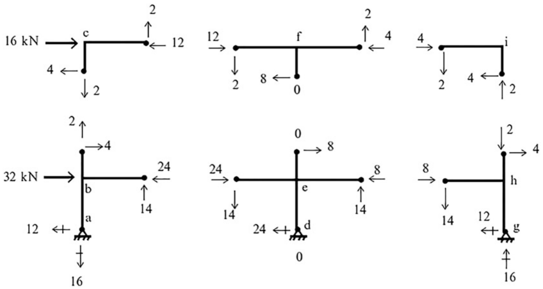
Fig. E11.1g Axial and shear forces (kN)
