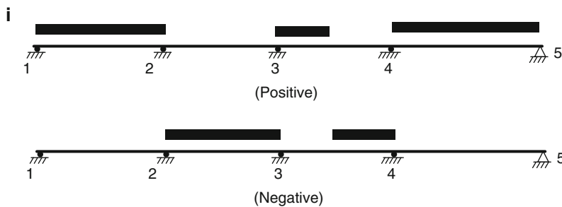
Fig. E13.1i Loading patterns for absolute maximum V_{1-1}
