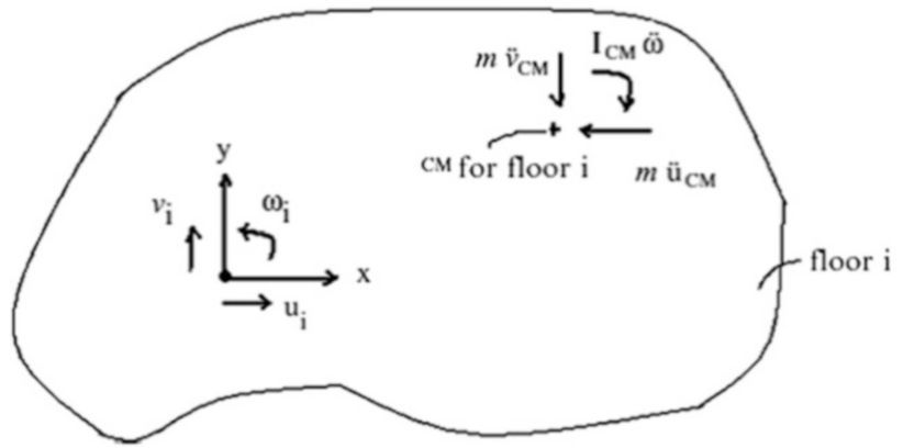
Fig. 14.21 Inertia forces for floor i
