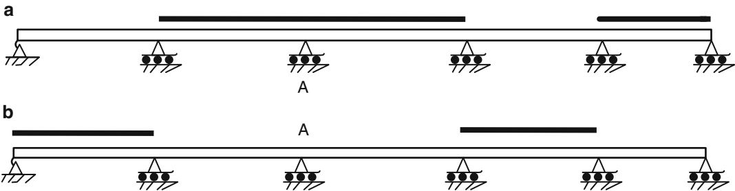
Fig. 13.3 Loading zones for moment at A. (a) Negative moment at A. (b) Positive moment at A
