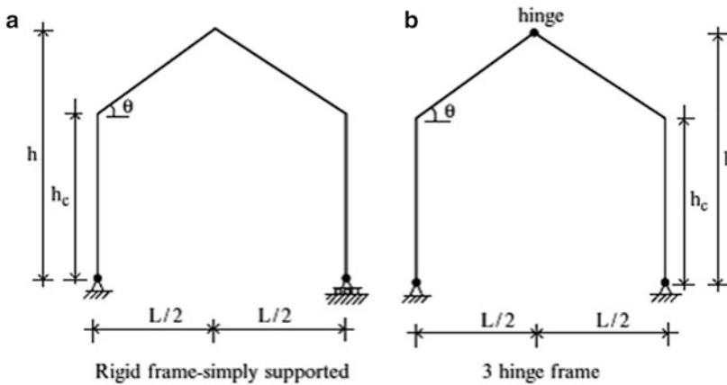
Fig. 4.16 Pitched roof frames
