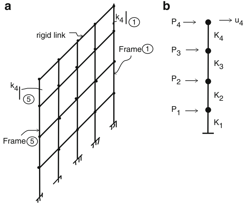
Fig. 14.26 Idealized building model. (a) Set of frames with rigid link. (b) Global loads and global story stiffnesses
