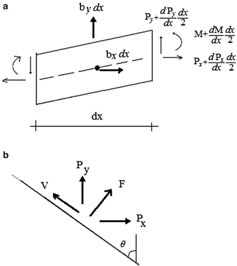
Fig. 10.33 (a) Differential element (b) Cartesian components
