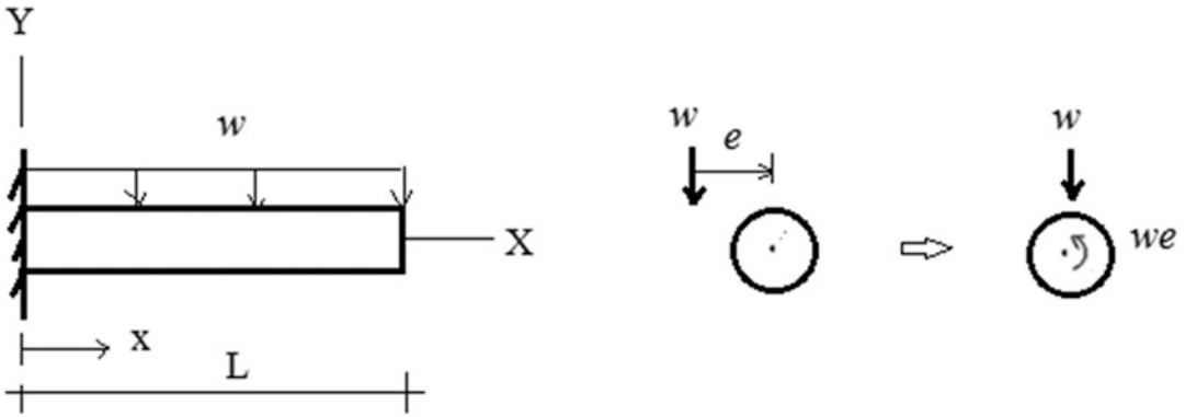
Fig. 3.36 Eccentrically loaded member
