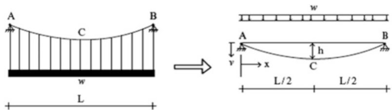
Fig. 5.13 Cable with a uniformly distributed loading
