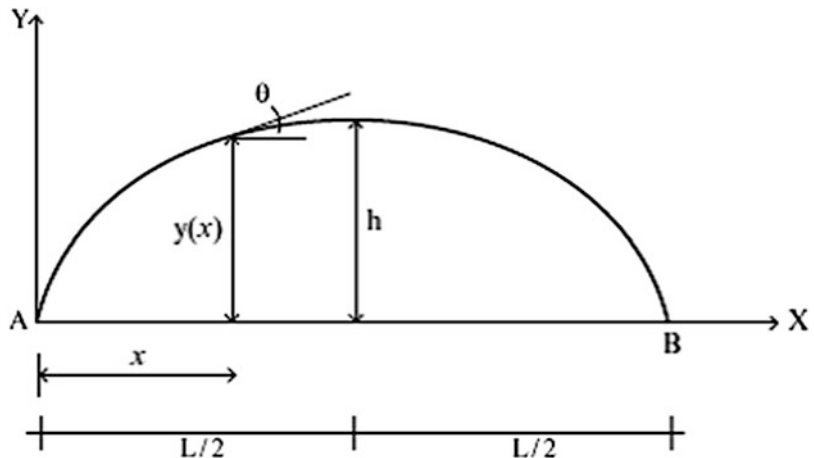
Fig. 6.17 Notation for parabolic shape function
