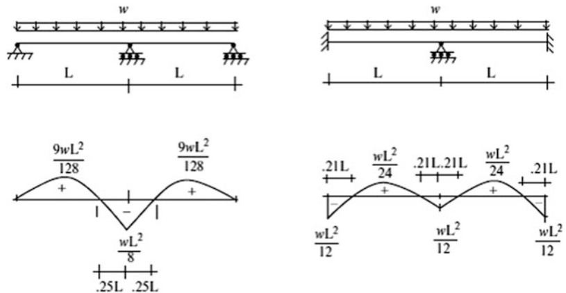
Fig. 11.2 Moment diagrams for two-span beams
