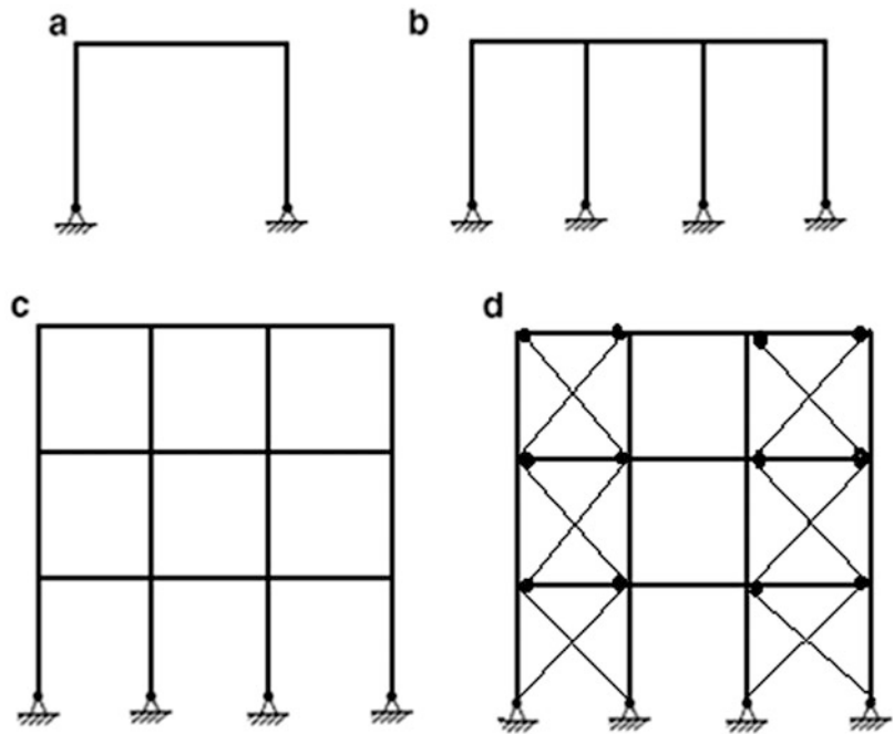
Fig. 4.1 Typical plane building frames. (a) Rigid portal frame. (b) Rigid multi-bay portal frame. (c) Multistory rigid frame. (d) Multistory braced frame
