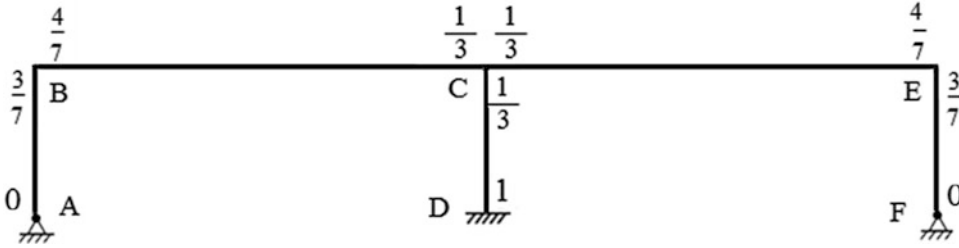
Fig. E10.15b Distribution factors
