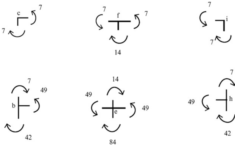
Fig. E11.1d Moments at the joints (kN m)
